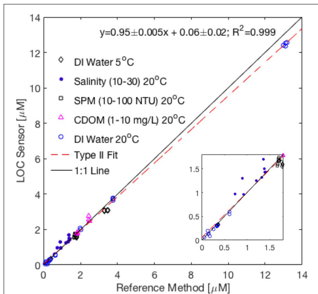
FIGURE 7 | Comparison of phosphate concentrations determined using Sensor 2 and values obtained using USEPA Reference method No 365.5 at the 17 exposure conditions tested as part of the Nutrient Sensor Challenge ( n = 62 ). Also included are reference and sensor measurements performed at the beginning of each day of testing, when the test tank was filled with deionized water (as low as 0.06 \mu\text{M PO}_4^{3-} ). Data from the highest phosphate concentration tested ( 60 \mu\text{M} ) are not shown nor included in the fit (see text for details). The dashed shows the Type II Linear Regression between sensor and reference method. The inset graph plots the same data at a reduced scale. DI, Deionized water; SPM, Suspended Particulate Matter; NTU, Nephelometric Turbidity Units; CDOM, Colored Dissolved Organic Matter.
