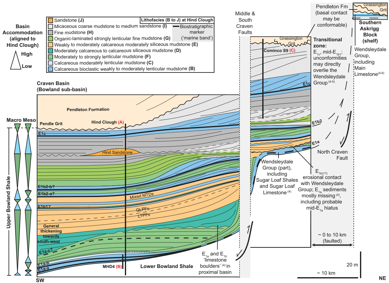
Fig. 18. Cross-section from the Askrigg Block (north-east) to Craven (Bowland) Basin (south-west), with extrapolated sedimentary facies observed at Hind Clough (A), MHD4 (B) and Cominco S9 (C). '1' Aitkenhead et al. , 1992; '2' Brandon et al. , 1998; '3' Kirby et al. , 2000; '4' Arthurton et al. , 1988; '5' Rowell & Scanlon, 1957; '6' Hudson, 1940. See text for Discussion and see Fig. 2 for transect position.
