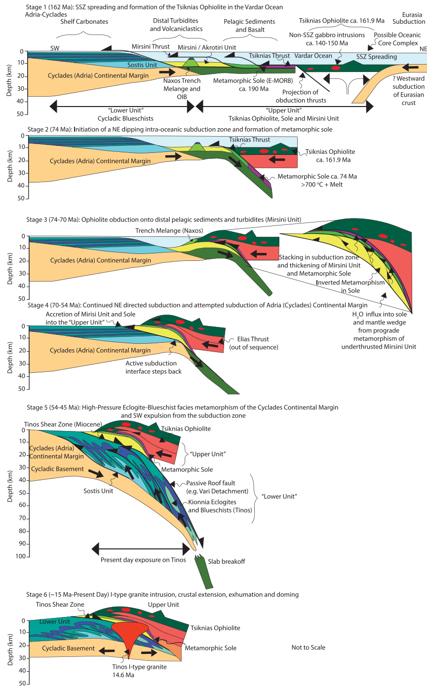
Figure 19. Tectonic model for the formation and emplacement of the Tsiknias Ophiolite, metamorphic sole, and subduction of the NE Cycladic continental margin. Stage 1: ~161.9 Ma: Tsiknias Ophiolite formation above a westward dipping subduction zone, preexisting ~190 Ma E-MORB crust to the SW which is the protolith to the metamorphic sole. Stage 2: ~74 Ma: Initiation of NE dipping subduction zone in ~90 Myr old oceanic crust and sole formation on the subduction interface due to conductive and shear heating. Stage 3: Ophiolite obduction and stacking of Mirisini Unit distal oceanic metasediments beneath the ophiolite. Stage 4: Detachment below the Mirisini Unit and main subduction thrust structurally steps backward. Continued subduction for 25 Myr before arrival of the Cycladic continental margin. Stage 5: Attempted subduction of the Cycladic continental margin at ~52–45 Ma causing high-pressure eclogite and blueschist-facies metamorphism of the Cycladic Blueschists and SW directed extrusion of the Cycladic Blueschists and stacking of the nappe pile. Top-to-NE shear fabrics are preserved at the top of the extruding slab and top-to-SW fabrics record internal thrusting within and at the base of the Cycladic Blueschist Unit. The highest-pressure rocks are preserved at the highest structural level of the Cycladic Blueschists (see Figures 2 and 3) and Laurent et al. (2016). Stage 6: 15 Ma: Present day: Onset of regional extension, I-type granite intrusion, exhumation of the Lower Unit and juxtaposition against the Upper Unit due to movement on the Tinos Shear Zone. E-MORB = enriched mid-ocean ridge basalt.
