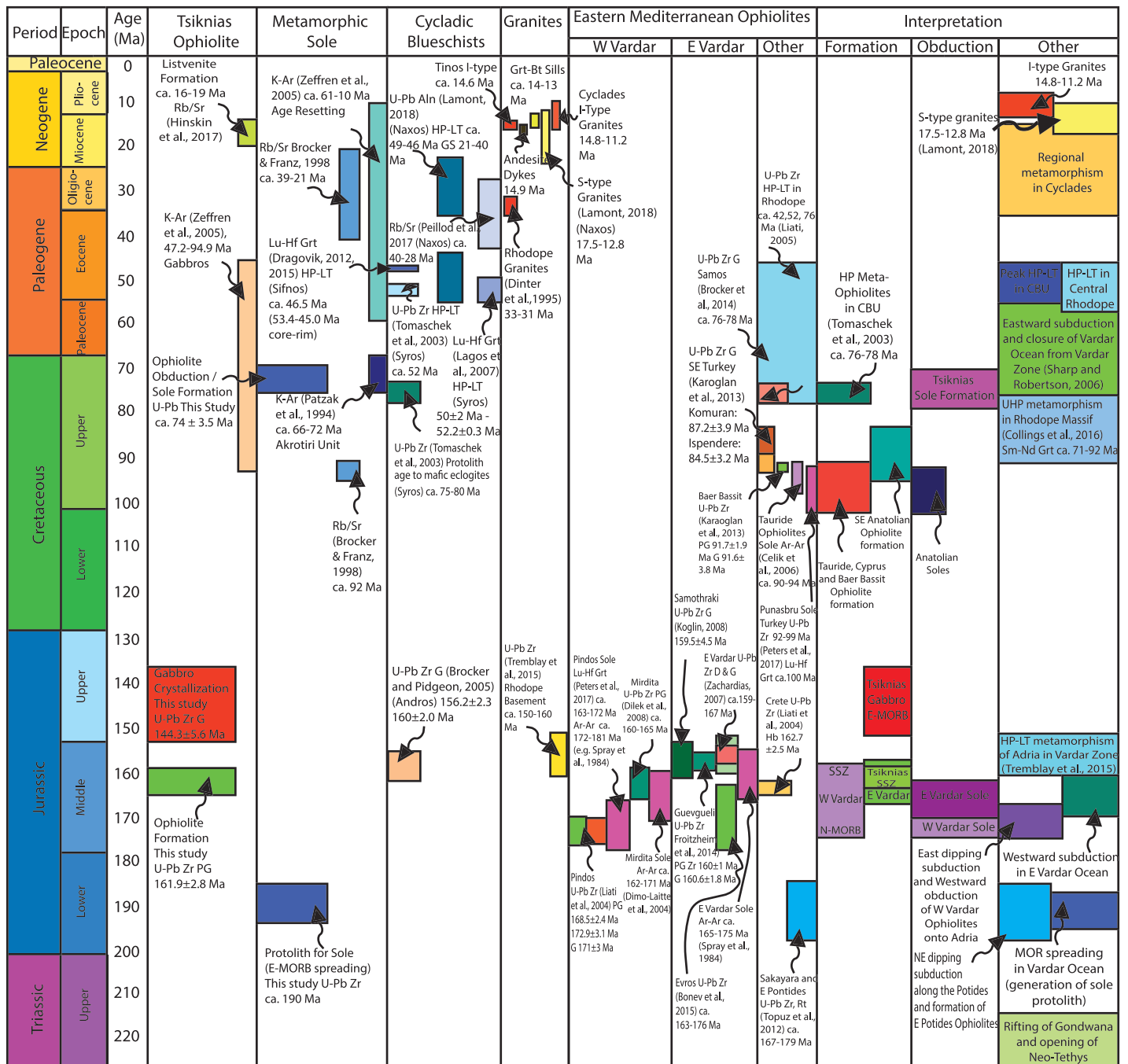
Figure 17. Annotated time chart for the Tsiknias Ophiolite and metamorphic sole with a compilation of literature age data from U-Pb, K-Ar, 40 Ar- 39 Ar, Rb-Sr, and Lu-Hf and Sm-Nd garnet ages. It includes data from granites, the Cycladic Blueschists, and other Eastern Mediterranean Ophiolites to help correlate the reported ages in this study.
