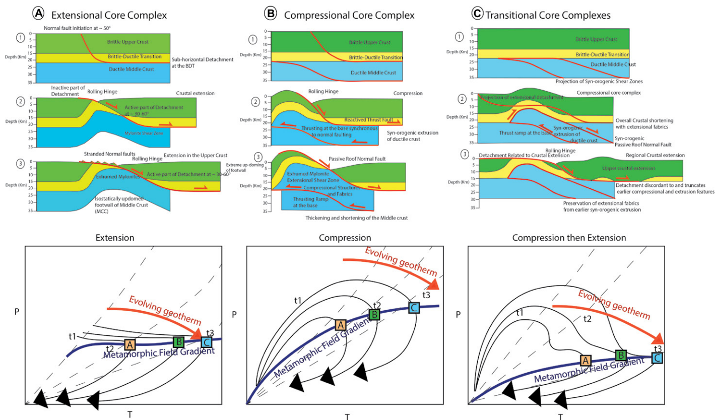
Figure 1. Schematic cartoons illustrating various tectonic models and pressure-temperature-time ( P-T-t ) paths associated with the formation of metamorphic core complexes (MCCs) (after Weller et al., 2013). The cogenetic suite of P-T-t paths is shown for three samples (A, B, and C), where the P-T loci of their respective T -max positions define the metamorphic field gradient, which is typically concave to the T -axis, polychronic, and at a steep angle to the P-T paths of an individual sample (England and Richardson, 1977; England and Thompson, 1984; Spear, 1993): (A) Classical cordilleran-style MCC formed by simple shear extension of the entire continental lithosphere and unroofing under a low-angle normal fault (e.g., Basin and Range). Predicted P-T-t path dominantly follows an isobaric heating excursion at lower pressure due to increased basal heating. BDT—brittle-ductile transition. (B) Compressional-type MCCs formed by doming above a thrust ramp at depth coeval with exhumation under a passive-roof normal fault (e.g., North Himalayan gneiss domes). These record a classical Barrovian type P-T-t path with heating to peak temperatures due to radiogenic heating. (C) Transitional MCC, where compression and crustal thickening cause metamorphism and early synorogenic extrusion followed by the switch to regional extension responsible for the last phase of heating and exhumation. This type is characterized by a classical Barrovian-type clockwise P-T-t path followed by an isobaric heating excursion upon the onset of extension.
