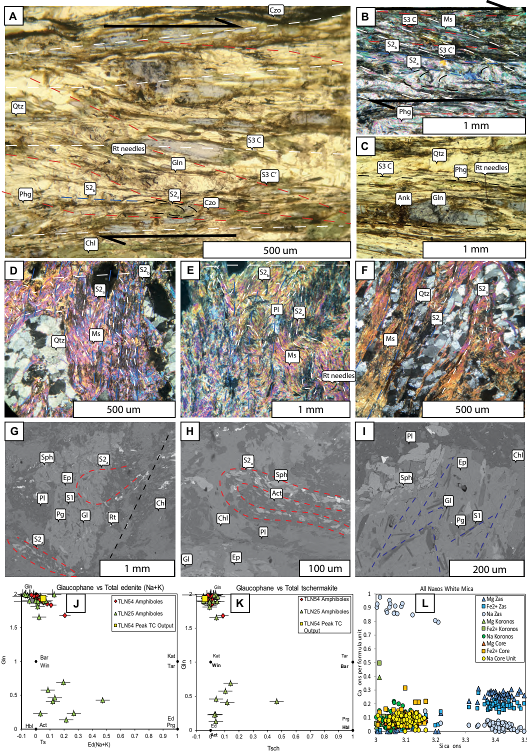
Figure 11. Representative photomicrographs and back-scattered electron images of Zas Unit microstructures and mineral chemistry. Mineral abbreviations follow Whitney and Evans (2010). (A–C) TLN54 (meta-tuff) glaucophane phengite schist displaying well-preserved glaucophanes aligned with S_1 top-to-the-NNE shearing fabrics, but also affected by S_3 top-to-the-NNE S-C' fabrics that affect both M_1 and M_2 assemblages. In lower-strain domains, S_{2a} and S_{2b} crenulation cleavages can be identified by folded bands of rutile needles, titanite phengite, and plagioclase, suggesting S_2 post-dated high-pressure conditions. (D–F) Quartz mica schist displaying well-developed S_2 microstructures including millimeter-scale isoclinal folds and S_{2a} crenulation cleavages, with no evidence for S_3 . This greenschist assemblage implies that S_2 fabrics also developed during M_2 . (G) TLN25 (Zas Unit) backscattered image showing calc-schist, where epidote traps earlier S_{2a} fabric, and micro-folding is defined by phengitic mica, actinolite, and titanite. Inclusions of glaucophane and paragonite in epidote represent M_1 conditions and outline S_1 fabrics. S_3 top-to-the-NNE extensional S-C' fabrics affect matrix assemblages including actinolite, chlorite, and plagioclase. (H) TLN25 backscattered image showing S_2 microfolds that is defined by grains of titanite that formed after peak M_1 conditions and predate greenschist-facies shearing. This implies that S_2 crenulation cleavages formed at upper-greenschist-facies conditions on the retrograde part of the pressure-temperature loop. (I) TLN25 close-up backscattered image of M_1 inclusions in epidote defined by glaucophane and paragonite, which preserve S_1 S-C shear fabric. Small inclusions of sphene are included in epidote, although coarse sphene grows externally. (J) Glaucophane vs. total edenite for Zas Unit samples plotting solely in the bottom left-hand corner diagnostic of low-temperature-high-pressure amphibole. TC output—Thermocalc output. (K) Glaucophane vs. total tschermakite for Zas Unit samples TLN54 and TLN25 showing the range from actinolite to glaucophane compositions, with TLN54 modeled glaucophane composition for comparison. (L) All Naxos white mica; note the distinctive trimodal population of data, where high Si (>3.4 pfu) represents high-pressure phengite solely within the Zas Unit, high Na (>0.9 pfu) is characteristic of paragonite, again only within the Zas Unit, and where Koronos and Core Units represent one mica population characteristic of Barrovian M_2 conditions.
