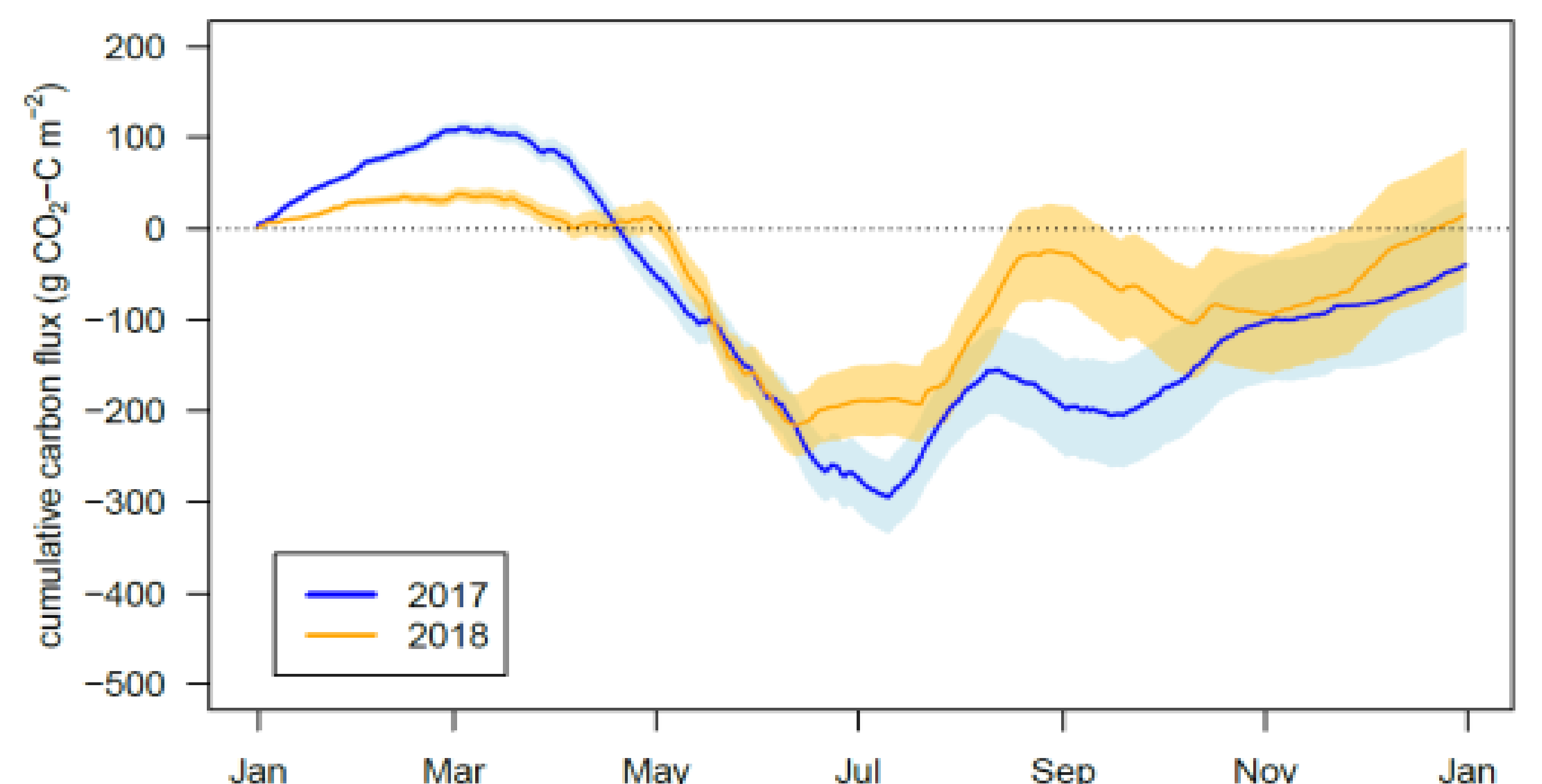
Figure 4. Cumulative net ecosystem C flux observed at an organically managed grassland on the Berkshire Downs (BD-EG) during 2017 and 2018.
