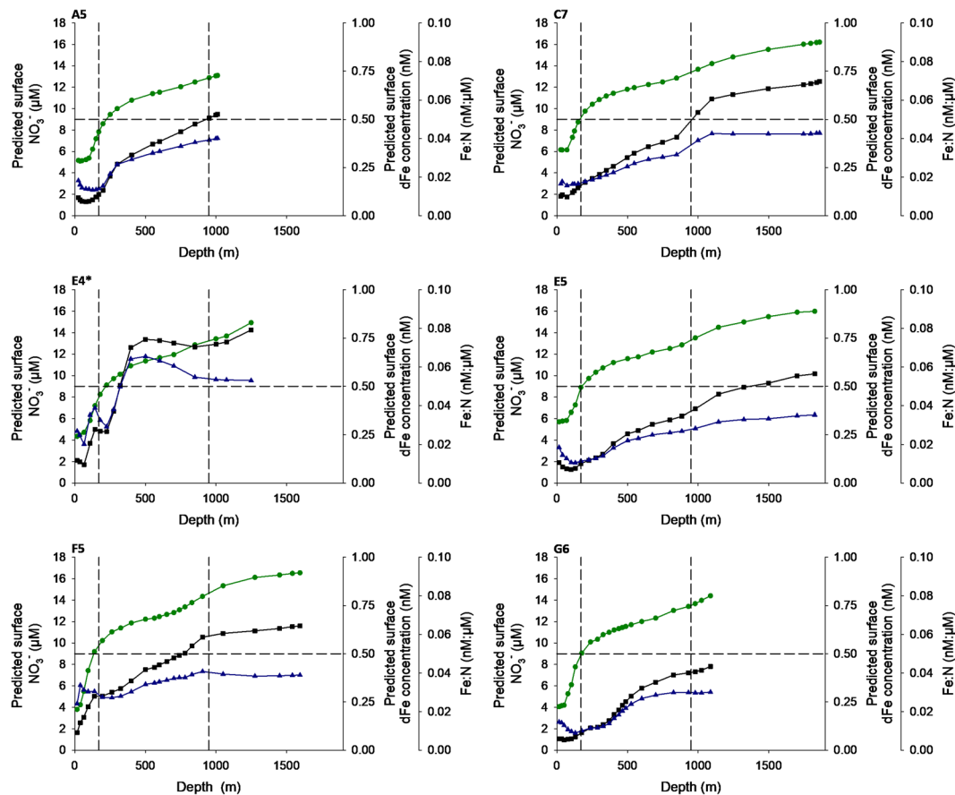
Figure 7. The estimated d\text{Fe}:\text{NO}_3^- surface stoichiometry resulting from winter mixing, calculated by integrating observed autumn concentrations from the surface to each depth sampled. This assumes a closed 1-dimension system. Vertical dashed lines provide an indication of the minimum and maximum winter mixing depths 11,39 . Observed winter (February) \text{NO}_3^- concentrations over the Hebridean shelf break are 10\text{--}11\ \mu\text{M} 57 and spring (April/May) d\text{Fe} concentrations are 0.16\text{--}0.64\ \text{nM} 15 . Horizontal dashed line indicates an \text{Fe}:\text{N} ratio of 0.05\ \text{nM}:\mu\text{M} , the lowest cellular content of phytoplankton observed during growth nutrient replete cultures 61,62 . *Shallow, iron rich intermediate nepheloid layer observed at station E4 results in an elevated d\text{Fe}:\text{NO}_3^- ratio (see Fig. S1).
