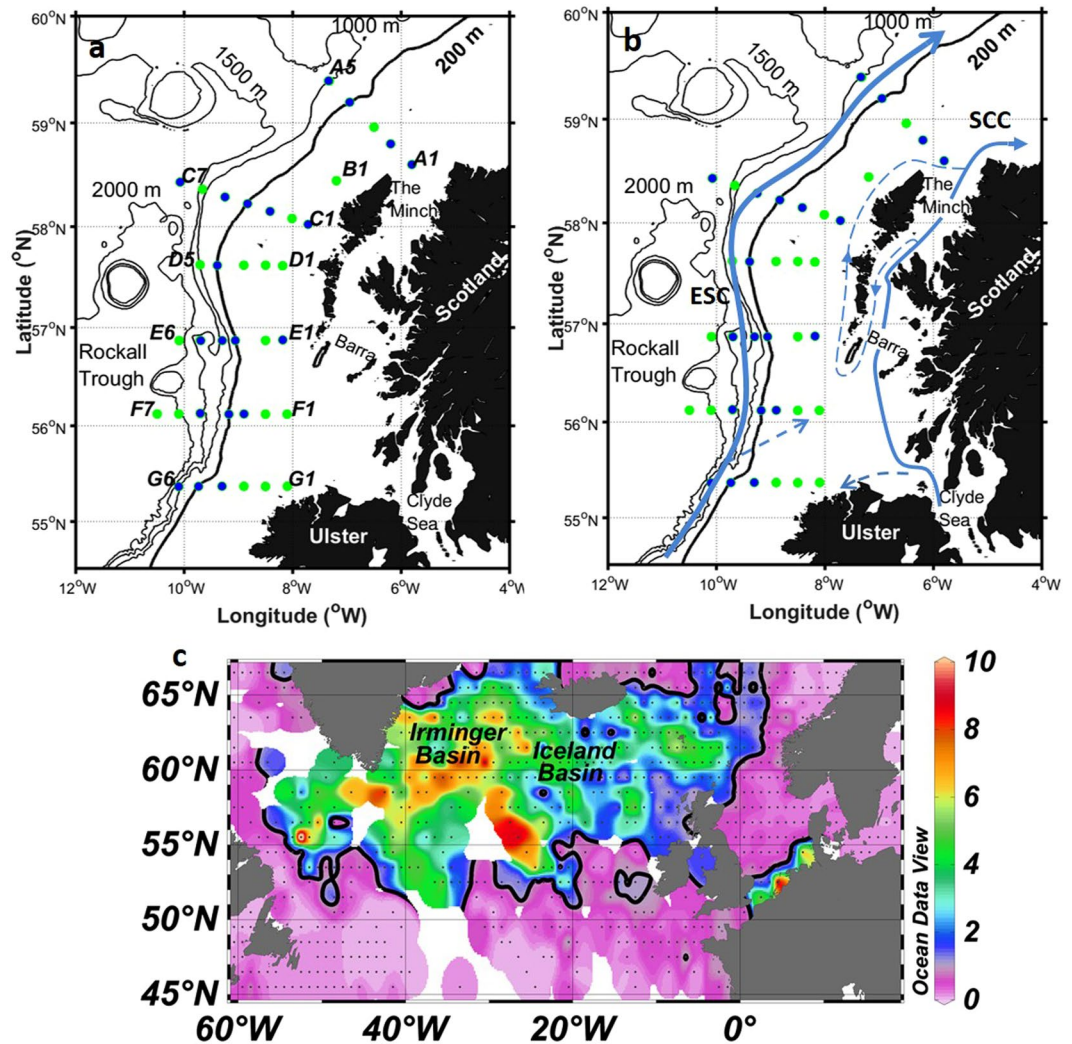
Figure 1. (A) Map of survey area denoting CTD sampling stations. Locations which included dissolved iron measurements are indicated by blue fill. (B) Map detailing the major currents and their approximate paths (ESC = European Slope Current, SCC = Scottish Coastal Current). (C) Climatology of summer surface nitrate concentrations ( \mu\text{M} ) in the sub-Arctic Atlantic from the World Ocean Atlas 79 . Solid black line indicates the 1 \mu\text{M} contour.
