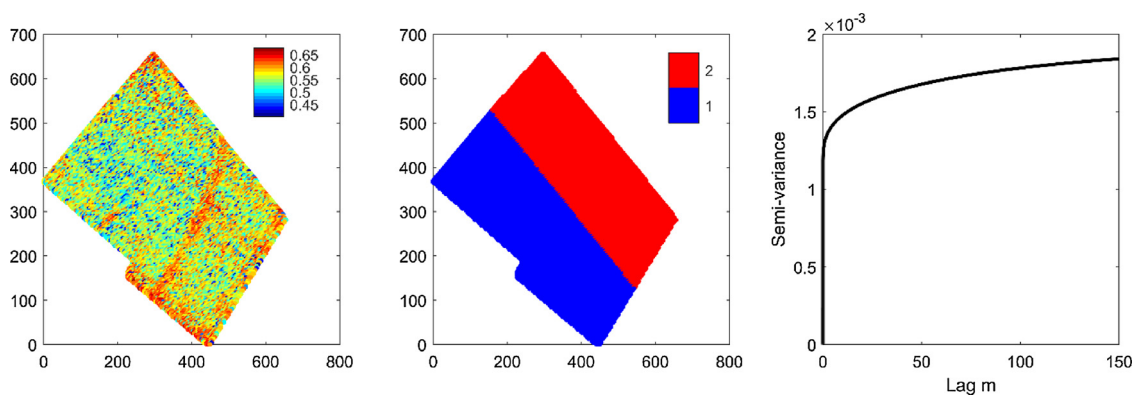
Fig. 12. (left) cleaned and aerial NDVI data from Experiment 1; (centre) experimental treatments; (right) estimated variogram. Coordinates are in m.
