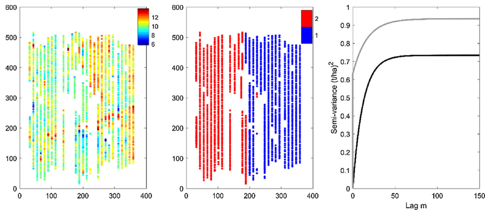
Fig. 4. (left) cleaned and rotated commercial yield monitor data from Experiment 1 ( t \text{ ha}^{-1} ); (centre) experimental treatments; (right) estimated variograms in direction of travel (black) and perpendicular to direction of travel (grey). Coordinates are in m.
