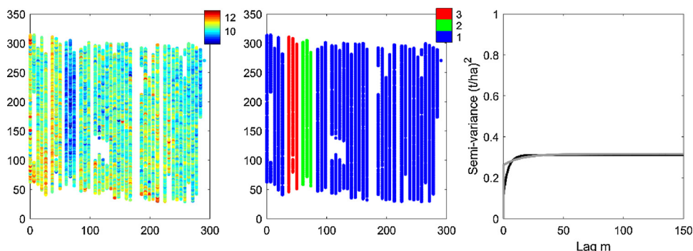
Fig. 7. (left) cleaned and rotated commercial yield monitor data from Experiment 4 ( t\ ha^{-1} ); (centre) experimental treatments; (right) estimated variograms in direction of travel (black) and perpendicular to direction of travel (grey). Coordinates are in m.
