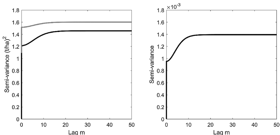
Fig. 9. (left) estimated variograms in direction of travel (black) and perpendicular to direction of travel (grey) for plot combine harvester yield monitor data from Experiment 5; (right) estimated variogram for handheld NDVI data from Experiment 5.
