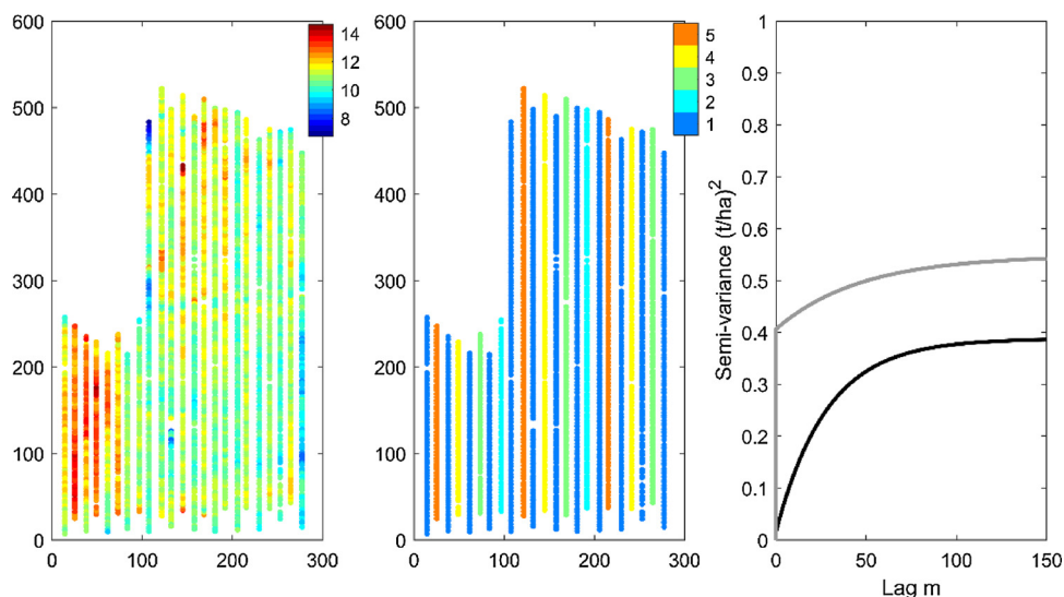
Fig. 5. (left) cleaned and rotated commercial yield monitor data from Experiment 2 ( t\ ha^{-1} ); (centre) experimental treatments; (right) estimated variograms in direction of travel (black) and perpendicular to direction of travel (grey). Coordinates are in m.
