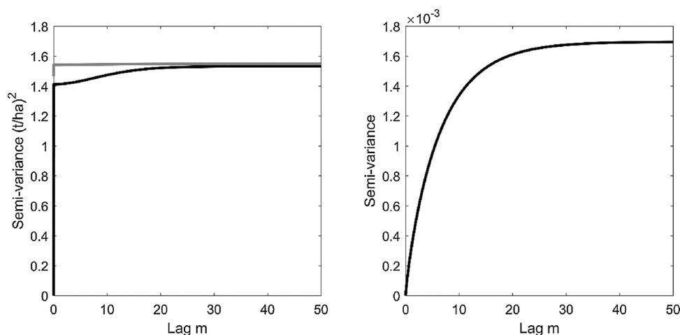
Fig. 11. (left) estimated variograms in direction of travel (black) and perpendicular to direction of travel (grey) for plot combine harvester yield monitor data from Experiment 6; (right) estimated variogram for handheld NDVI data from Experiment 6.
