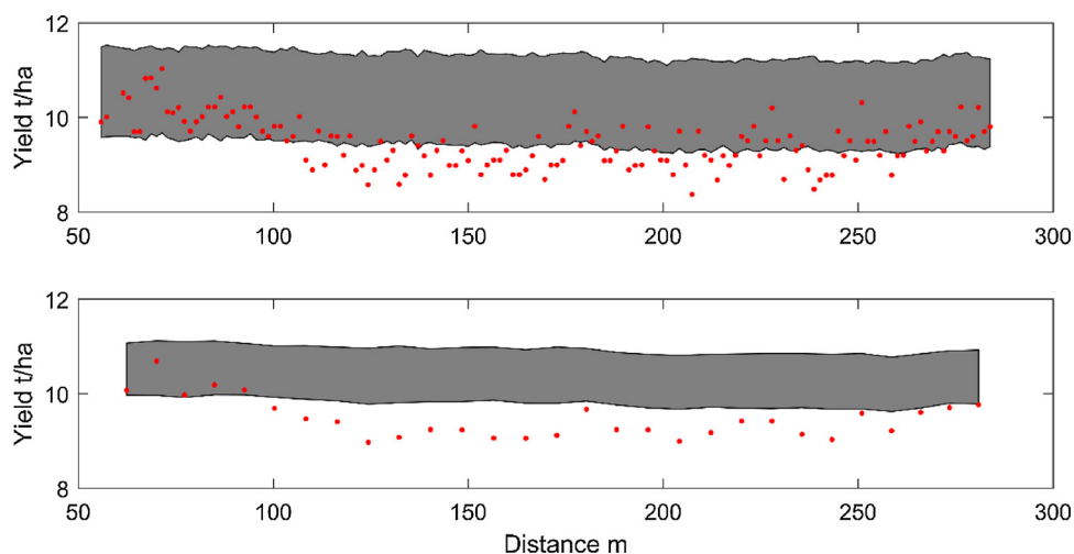
Fig. 13. Ninety percent prediction interval of yield at sites adjacent to treatment boundary under the model for the standard treatment (shaded area) and observed values at these sites under treatment 2 (red) for Experiment 4. Upper plot shows individual yield measurements and predictions whereas lower plot shows averages of five measurements.
