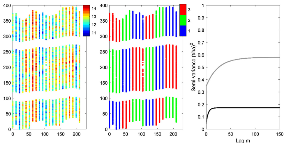
Fig. 6. (left) cleaned and rotated commercial yield monitor data from Experiment 3 ( t\ ha^{-1} ); (centre) experimental treatments; (right) estimated variograms in direction of travel (black) and perpendicular to direction of travel (grey). Coordinates are in m.
