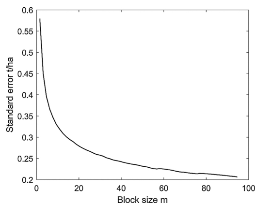
Fig. 14. Standard deviation of predictions of yield at sites adjacent to treatment boundary under the model for the standard treatment against the length of the block over which they are averaged.
