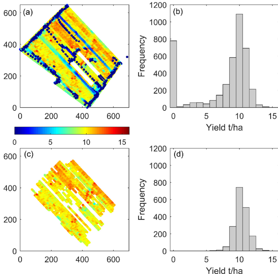
Fig. 2. (a) scatter plot of raw commercial yield monitor data from Experiment 1 (t/ha); (b) histogram of raw commercial yield monitor data from Experiment 1; (c) scatter plot of cleaned commercial yield monitor data from Experiment 1; (d) histogram of cleaned commercial yield monitor data from Experiment 1.
