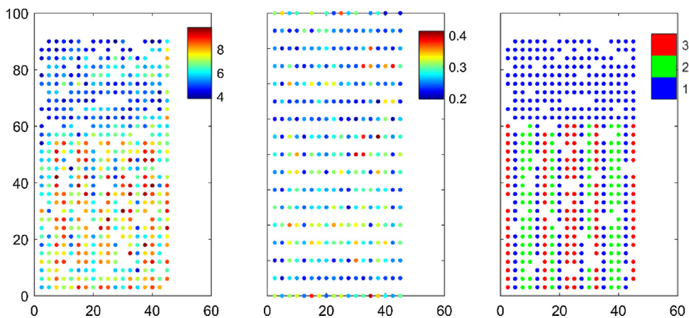
Fig. 8. (left) cleaned and rotated plot combine harvester yield monitor data from Experiment 5 ( t\ ha^{-1} ); (centre) cleaned and rotated handheld NDVI data from Experiment 5 (right) experimental treatments. Coordinates are in m.
