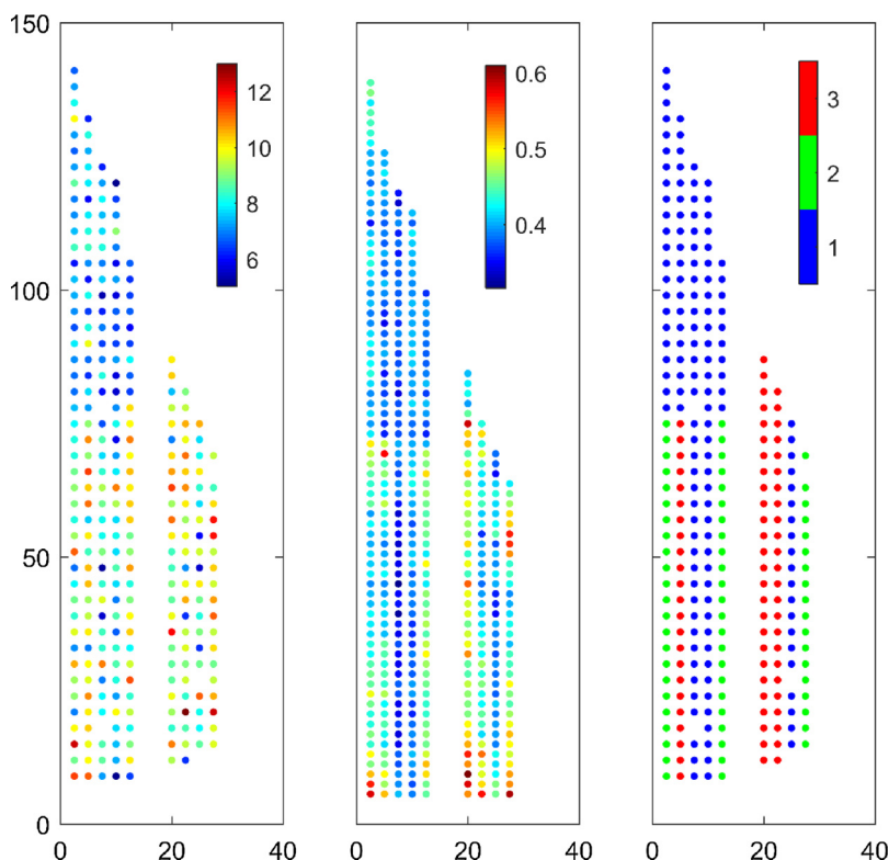
Fig. 10. (left) cleaned and rotated plot combine harvester yield monitor data from Experiment 6 ( t\ ha^{-1} ); (centre) cleaned and rotated handheld NDVI data from Experiment 6 (right) experimental treatments. Coordinates are in m.
