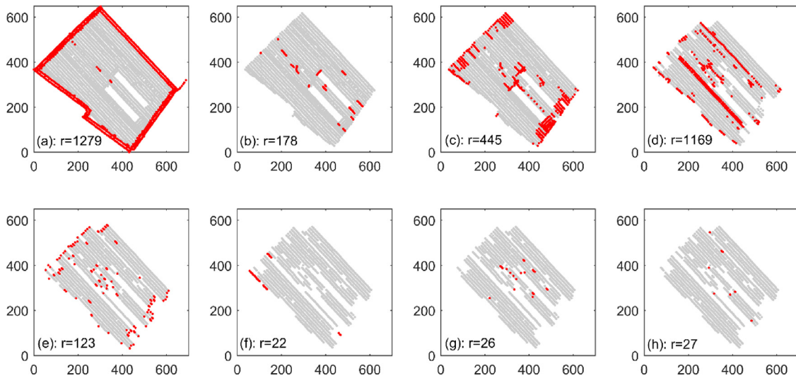
Fig. 3. Removed yield monitor observations (red dots) and remaining observations (grey dots) by the following filters (a) flagged by operator, (b) combine harvester velocity, (c) direction of travel, (d) already harvested location, (e) break in signal, (f) yield by line, (g) global threshold on yield and (h) local yield outliers. ‘r’ value indicates number of observations removed and the total number of observations was 4524. Coordinates are in m.
