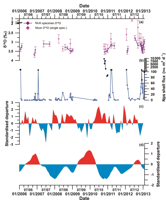
Figure 10. (a) Multi-specimen (purple) and single-specimen (pink) mean \delta^{18}\text{O}_{\text{np}} (error bars show \pm 1\text{SD} ). (b) Total Nps flux (black diamonds show statistically significant outliers, defined by interquartile range). (c) Southern Annular Mode (SAM) index and (d) El Niño–Southern Oscillation (ENSO) index. The SAM index is based on the departure from the zonal means between 40 and 65° S (Marshall, 2003). Red sections show positive SAM, and blue sections show negative SAM. The ENSO index is based on the departure from the 1950–1993 reference period (Wolter and Timlin, 2011). Red sections show El Niño-like conditions, and blue sections show La Niña-like conditions. Note the co-variation between positive SAM and La Niña-like conditions; negative SAM and El Niño-like conditions; and the strong positive SAM, La Niña and high Nps flux in 2010.
