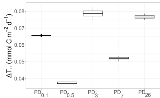
Figure 6. Development of \Delta T_{..} ( \text{mmol C m}^{-2} \text{d}^{-1} ), i.e., the difference in “total system throughput” T_{..} outside plough tracks compared to inside plough tracks, over time. \text{PD}_{0.1} corresponds to 0.1-year post-disturbance, \text{PD}_{0.5} is 0.5-year post-disturbance, \text{PD}_3 is 3-year post-disturbance, \text{PD}_7 is 7-year post-disturbance, and \text{PD}_{26} is 26-year post-disturbance event.
