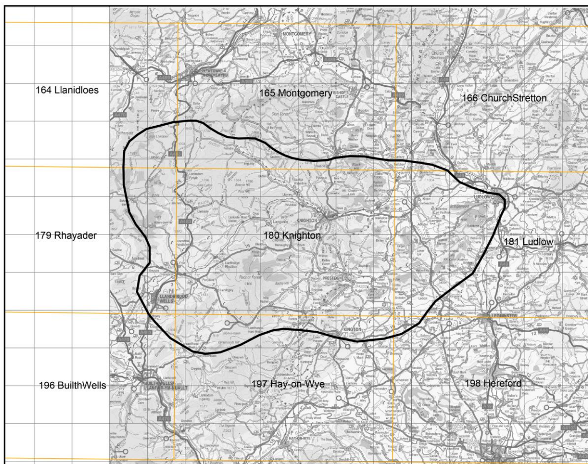
Figure 1 Extent of the approximate region covered by the scoping report showing the adjacent 1:50 000 series geological maps
