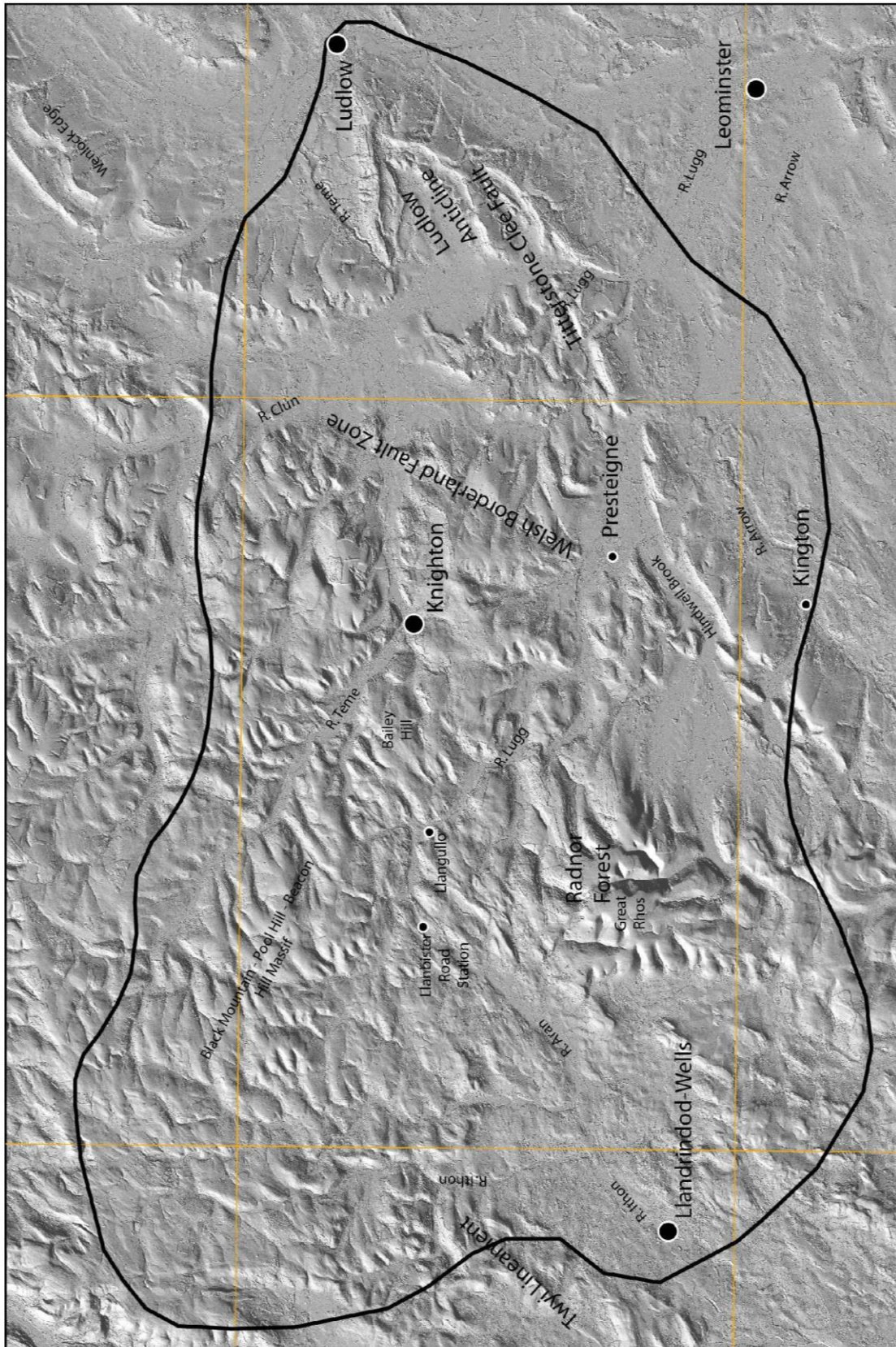
Figure 3. The physiography of the Knighton district and environs (hillsshade NextMap digital terrain model data).
