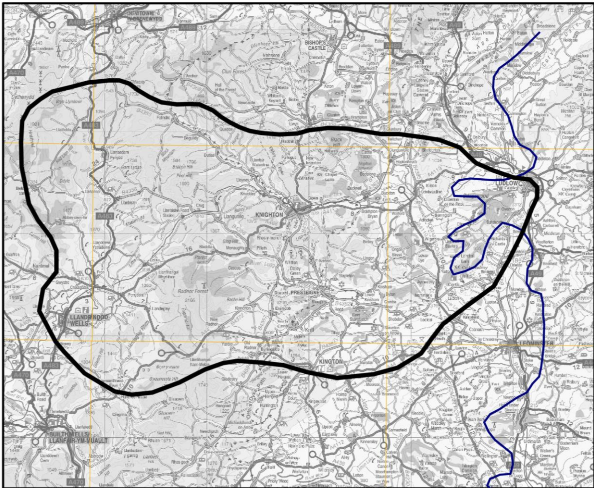
Figure 4. The current interpretation of the Devensian limit in the Knighton area.
