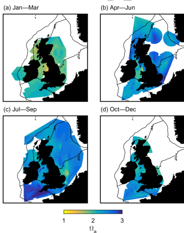
Figure 15: Aragonite saturation ( \Omega_a ) calculated from SSB bottle DIC and TA.
