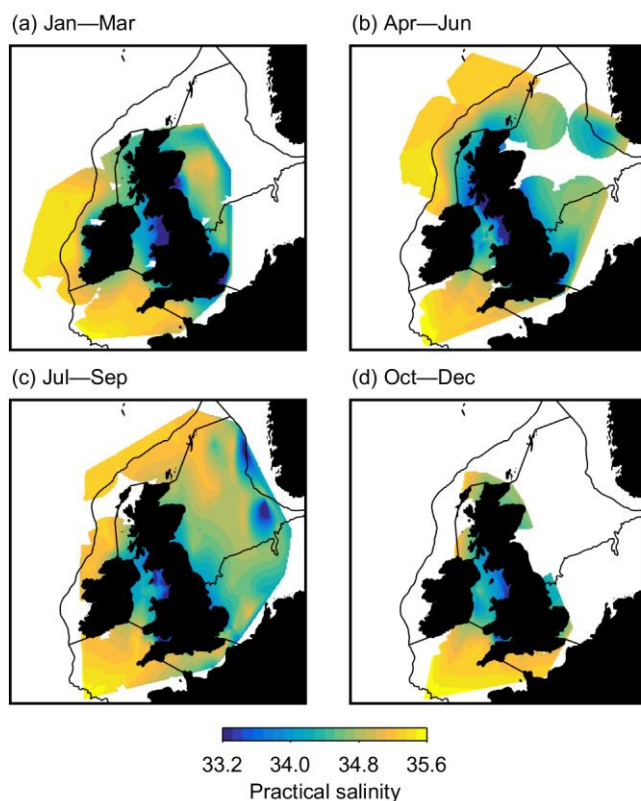
Figure 3: Seasonal maps of sea surface salinity (SSS) as practical salinity, using sensor data taken at the point of sampling on the SSB surveys.
