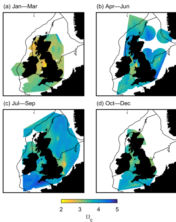
Figure 14: Calcite saturation ( \Omega_c ) calculated from SSB bottle DIC and TA.
