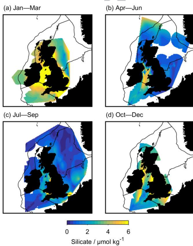
Figure 5: Seasonal maps of silicate concentrations, from SSB bottle samples.
