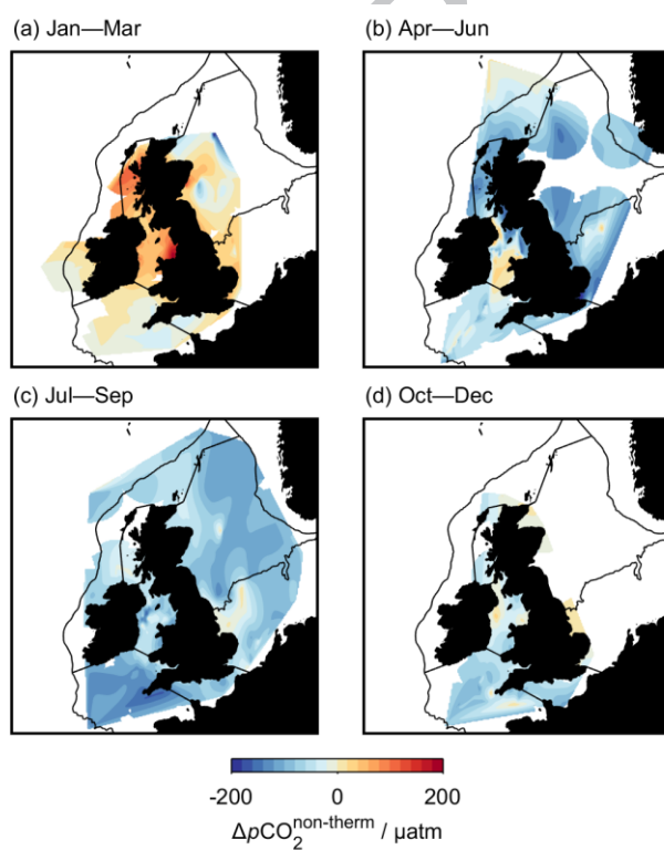
Figure 13: The non-thermal component of the change in pCO 2 (calculated following Takahashi et al., 2002 as the residual between the total and thermal component of change).
