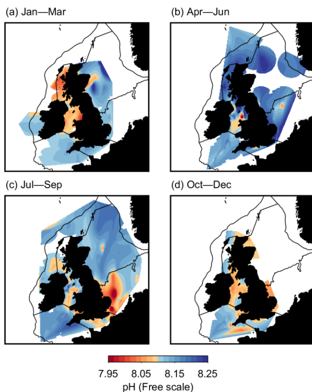
Figure 9: pH (freescale), calculated from bottle samples analysed for DIC/TA (using
