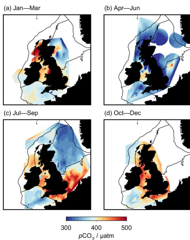
Figure 8: Surface p\text{CO}_2 , calculated from bottle samples analysed for DIC/TA (using \text{CO}_2\text{SYS} ) and measured p\text{CO}_2 from underway systems on the RRS Discovery and RV Cefas Endeavour (2014-2015).
