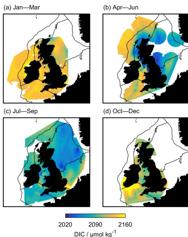
Figure 7: Dissolved Inorganic Carbon (DIC) measurements, from SSB bottle samples.
