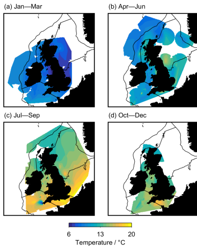
Figure 2: Seasonal maps of sea surface temperature (SST), using sensor data taken at the point of sampling on the SSB surveys. Figures 2-9, 12-15 are all mapped from 48 to 62°N, 16°W to 8°E showing winter (Jan-Mar), spring (Apr-Jun), summer (Jul-Sep) and autumn (Oct-Dec).
