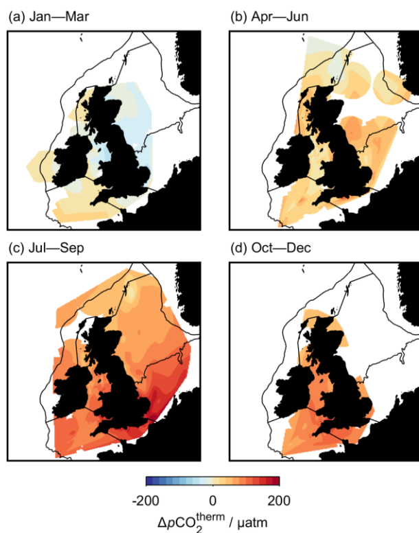
Figure 12: The thermal component of the change in pCO 2 calculated following Takahashi et al. (2002).
