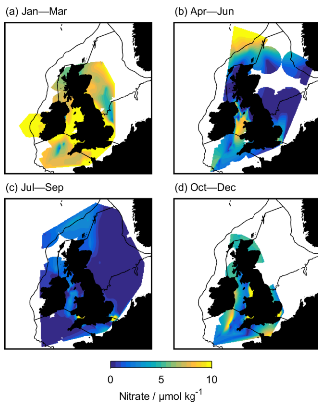
Figure 4: Seasonal maps of sea surface nitrate concentrations, from SSB bottle samples.
