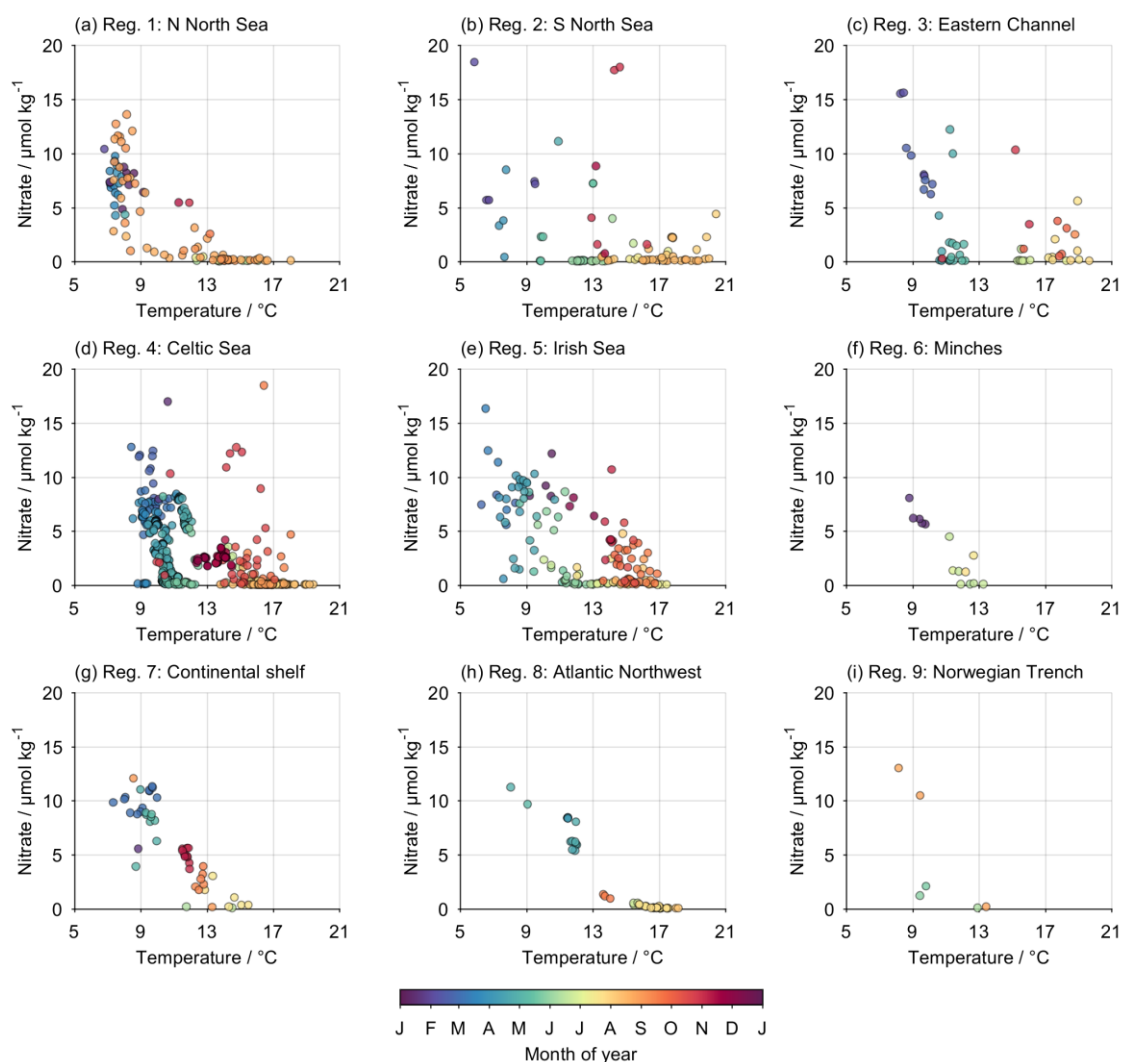
Figure 10: Measured nitrate concentrations and sea surface temperature for each month and region.
