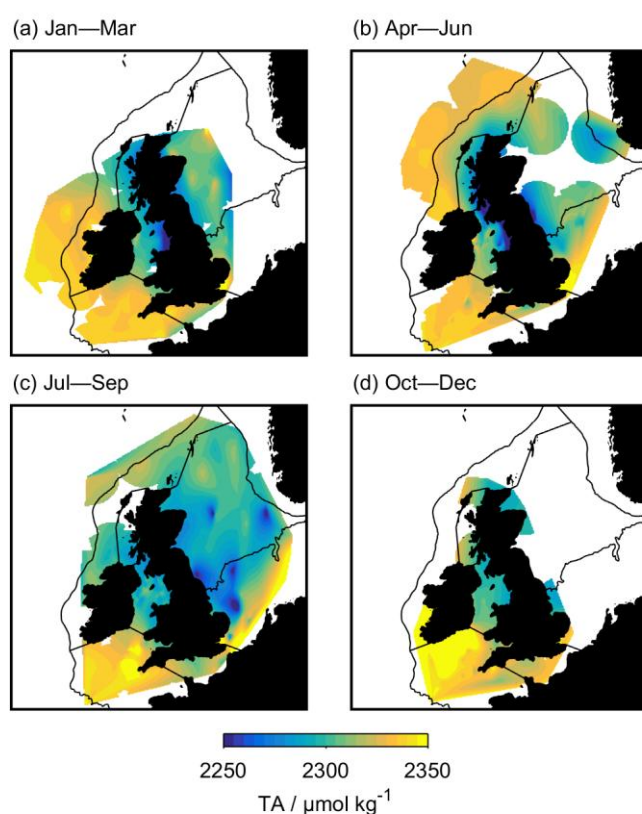
Figure 6: Seasonal maps of total alkalinity (TA) measurements, from SSB bottle samples.
