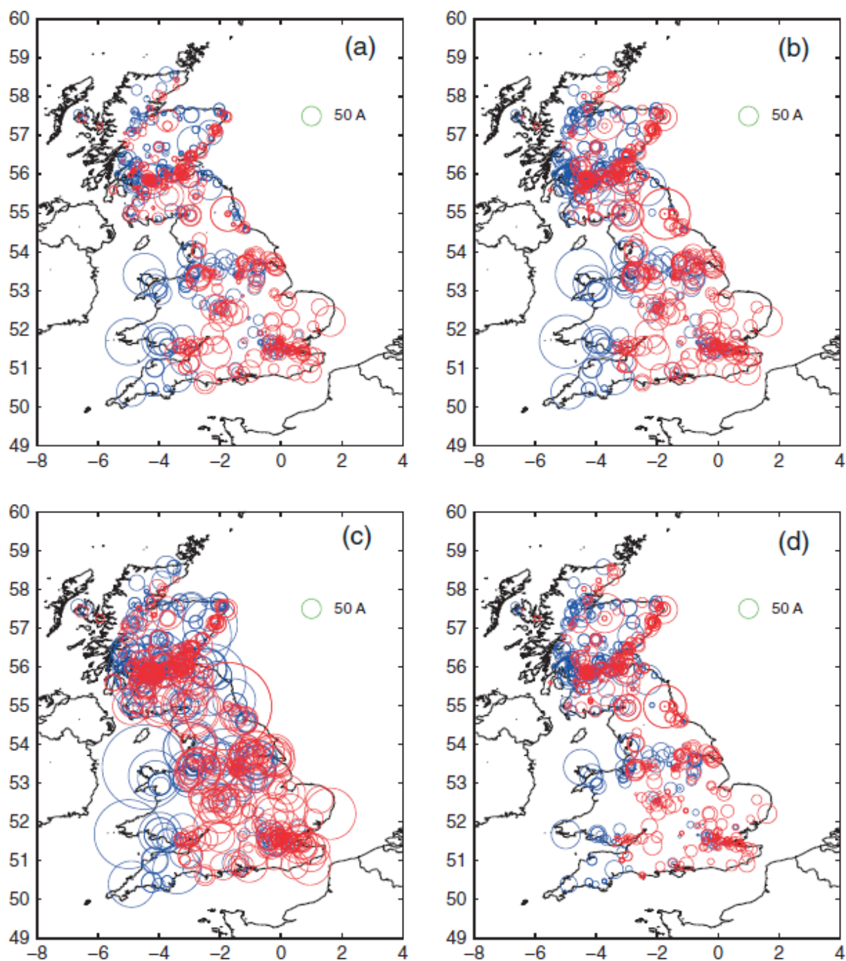
Figure 2-15: Snapshots of GIC in the National Grid GB high-voltage network due to an extreme storm scenario (approximately a factor of 5) of the 30 October 2003 geomagnetic storm (due to an electric field with a period of 120 s). (a) Time: 19.30 h, (b) Time: 20.50 h, (c) Time: 21:20 h, and (d) Time: 22:50 h (see Figure 2-5). Blue indicated GIC directed into the grid, red indicates GIC into the ground. Circle size represents size (relative to scale). Note that many sites host multiple transformers.
