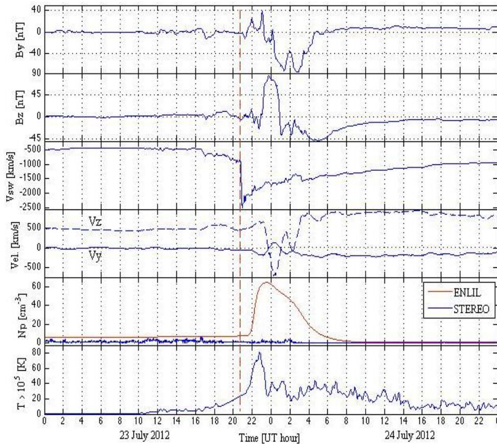
Figure 4-3: Solar wind in-situ observations from the STEREO-A spacecraft. From top to bottom are: the IMF B_y , IMF B_z , plasma bulk speed ( V_{sw} ), the velocity V_y (solid) and V_z (dashed) components, the solar wind density ( N_p ) and the temperature (Temp). Note that the density (red trace) is derived using the WSA-ENLIL 3-D MHD heliosphere model due to challenges in extracting the PLASTIC density data.
