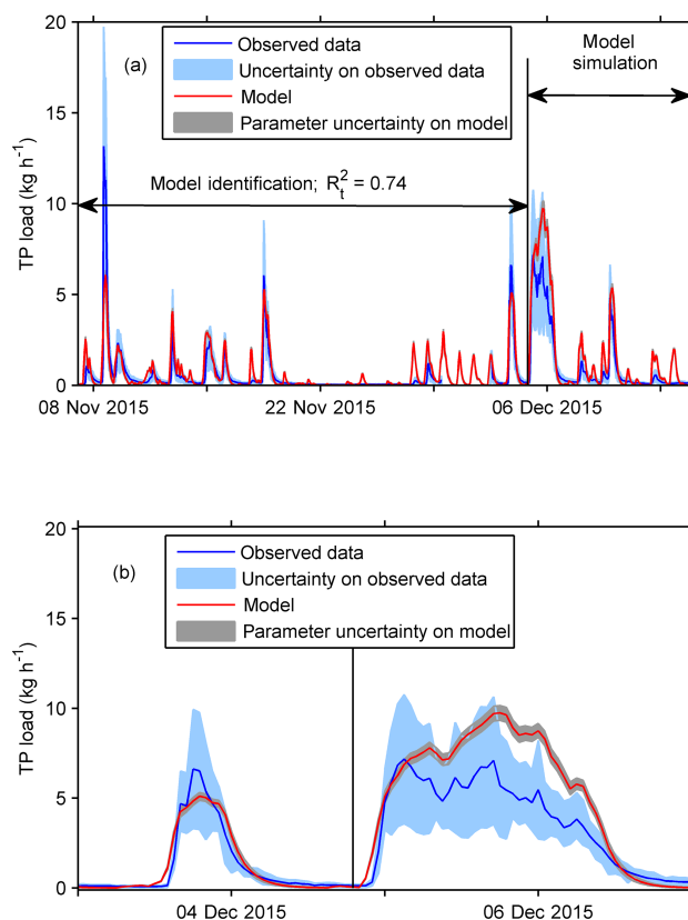
Figure 4. Observed and modelled total phosphorus (TP) load (a) and zoomed section of the same (b) in Newby Beck, Eden, during November 2015, with the same model used to estimate TP load during Storm Desmond 5–6 December 2015. The blue band indicates the 95 % uncertainty bounds on the measurement data. The grey band indicates the 95 % confidence limits on the parameter uncertainty. Total model predictive uncertainty (including the residual uncertainty) is larger than parametric uncertainty and would enclose the observations most of the time.
