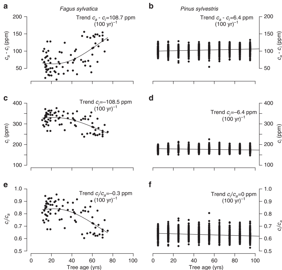
Fig. 4 Developmental trends in gas-exchange regulation diagnostics for Fagus and Pinus . a, b show air-to-leaf CO 2 difference ( c_a - c_i ), c, d show leaf internal CO 2 ( c_i ) and e, f show the ratio of leaf-to-air CO 2 ( c_i/c_a ) plotted against tree age. These values are calculated from the average \delta^{13}\text{C} (see Methods section for formulas) of the five outermost rings across a range of trees differing in tree age (for Fagus ) or from sub-fossil trees (for Pinus , Helama et al. 39 ). In both cases, age trends were controlled for changing CO 2 levels. a, c and e show results for Fagus and b, d and f for Pinus
