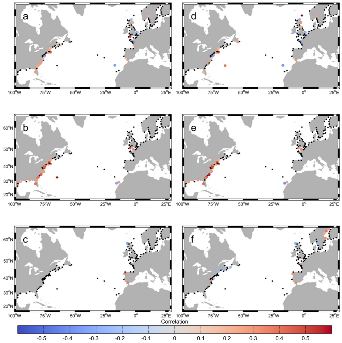
Figure S6. As Figure S4 but for NIÑO3.
