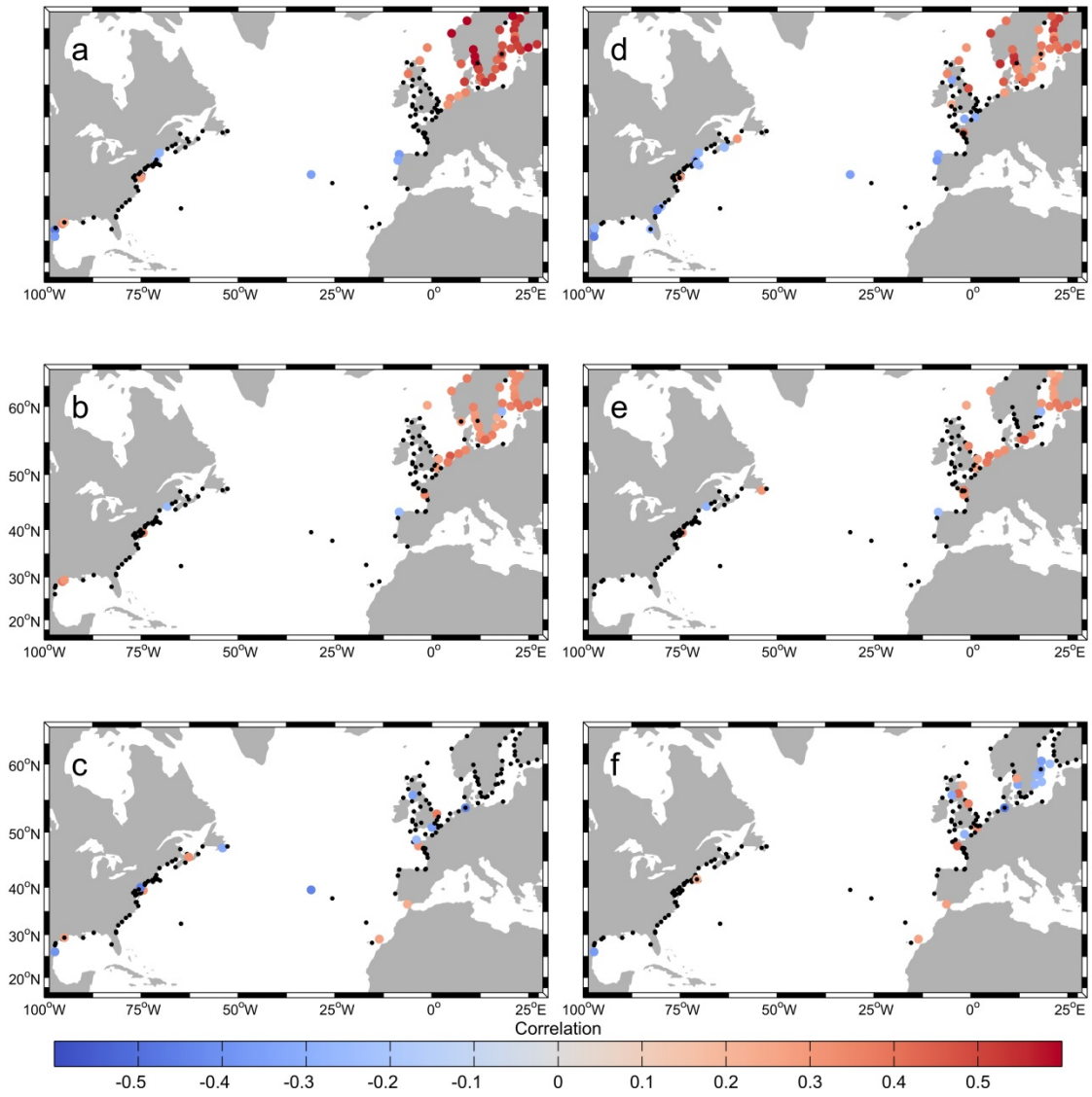
Figure S5. As Figure S4 but for AO.
