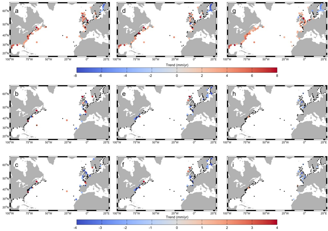
Figure S2. As in Figure 5 but for 99.9th percentile.
