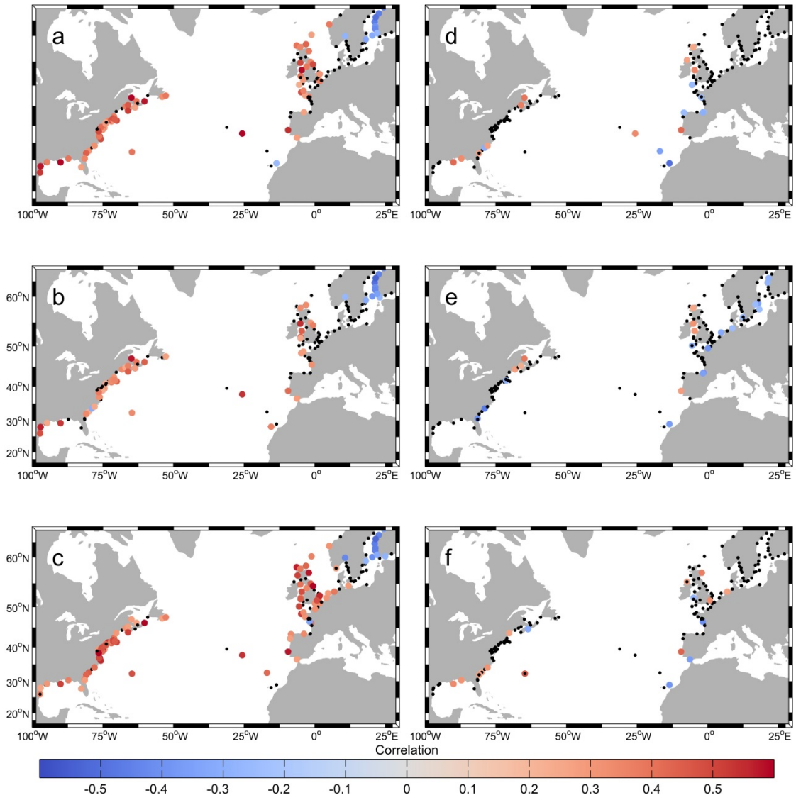
Figure S8. As Figure S4 but for AMO.
