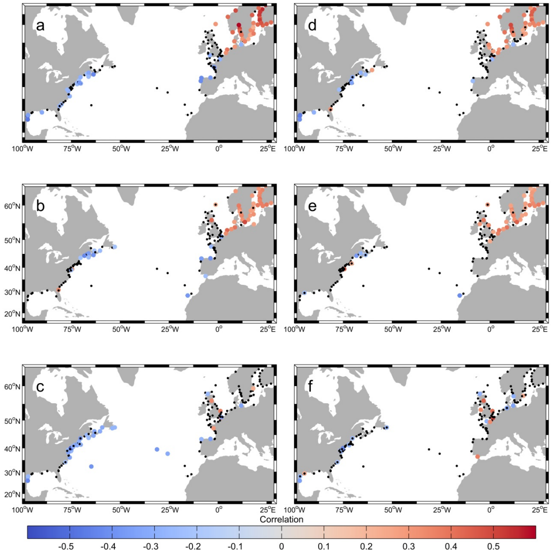
Figure S4. As in Figure 8 but for skew surges.
