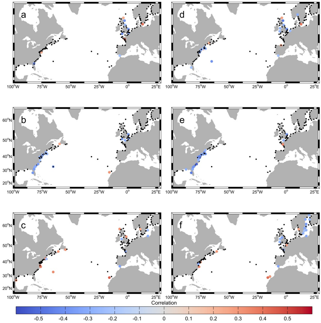
Figure S7. As Figure S4 but for SOI.
