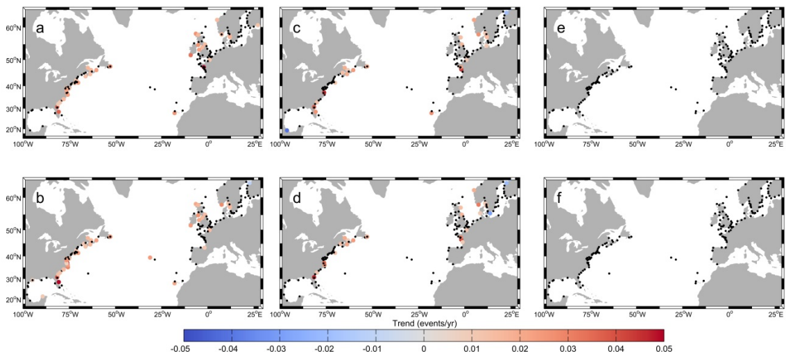
Figure S3. As in Figure 6 but for 99.9th percentile.
