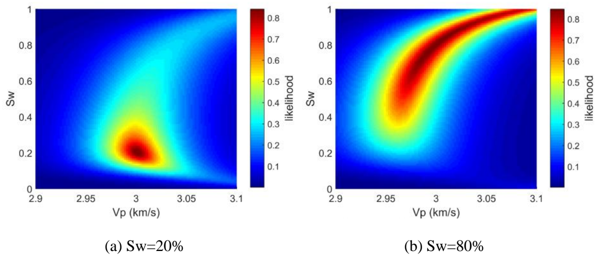
Figure 15. The likelihood function of water saturation and P-wave velocity at fixed reservoir thickness of 30 meters. (a) 20% water case. (b) 80% water case.
