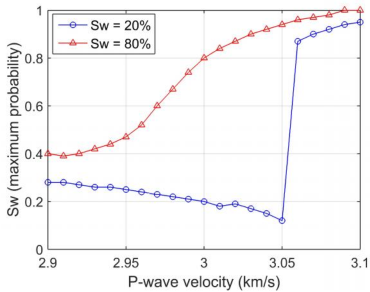
Figure 14. Sw with maximum posterior probability versus varying well-log P-wave velocities. The 20% water saturation case is indicated by blue circle, and the 80% water saturation case is labelled with red triangle. The true P-wave velocity is 3 km/s.
