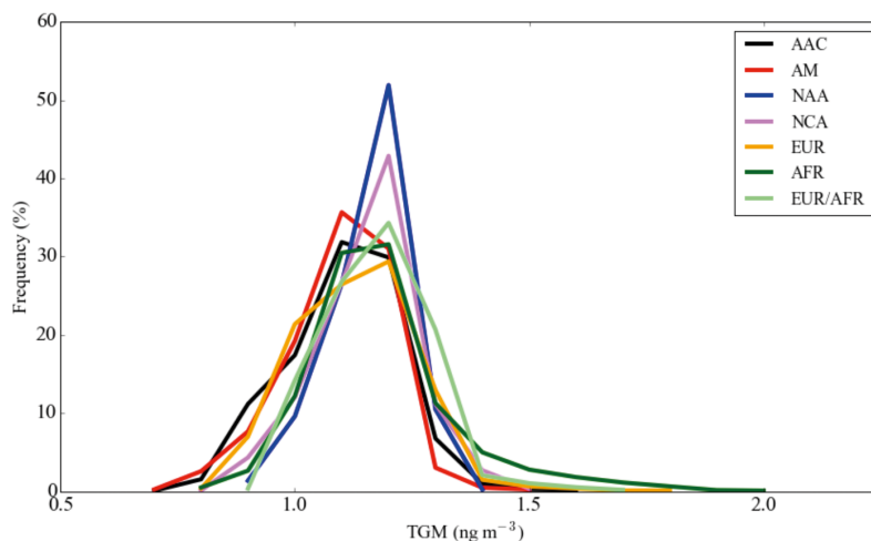
Figure 6. Histograms of observed TGM classified by air mass for the full 2011–2015 dataset.
