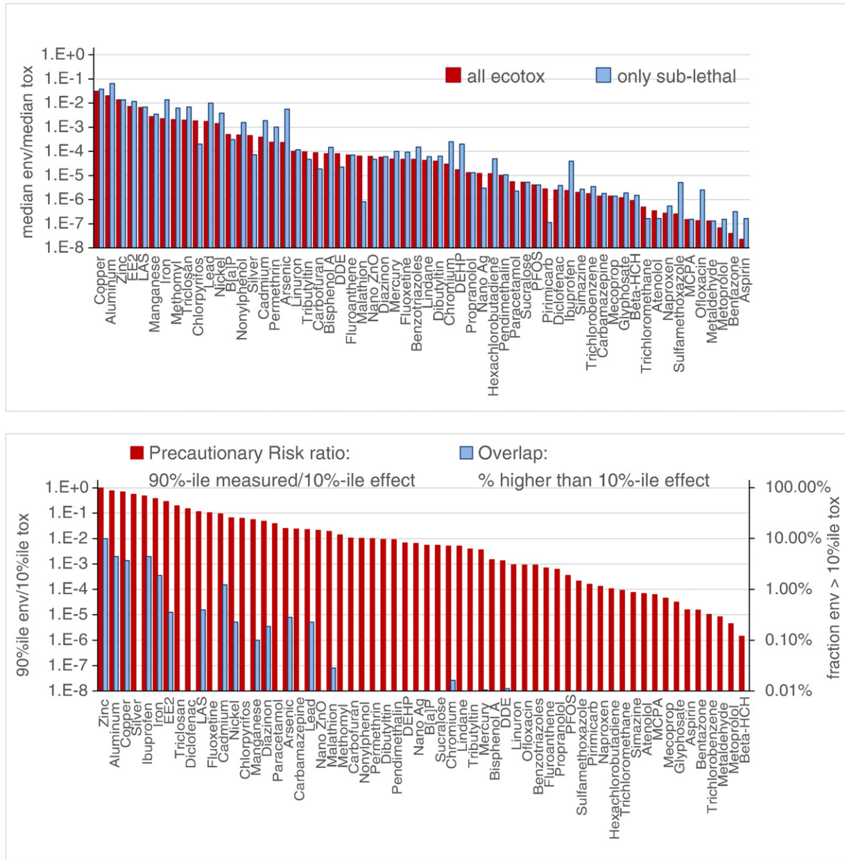
Fig. 3. Risk ranking of all 60 chemicals in tier 2. Top: based on the ratio of the median environmental concentrations versus the median of all ecotoxicity data, compared with the ratios if only the sub-lethal ecotoxicity data are used. Bottom: Assessing the potential impact on UK aquatic wildlife by either comparing the ratio of the highest 90%ile environmental data with the lowest 10%ile ecotoxicity data or by investigating what percentage of environmental measurements are above the 10%ile ecotoxicity data point. Only UK measured data since 2000 were considered. Note the same data are plotted on a natural scale and larger format as Fig. S2.
