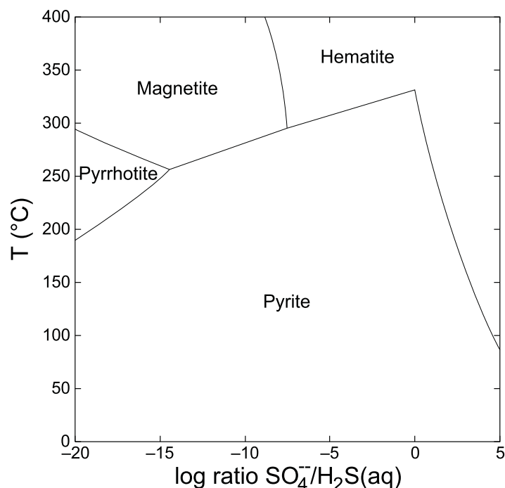
Figure 6. The stability of iron phases at 500 bar, \log \text{SO}_4^{2-} activity = -3 , \log \text{Cl}^- activity = -0.5 , \text{O}_2 activity is expressed as \text{SO}_4^{2-}/\text{H}_2\text{S} . The availability of pyrite and pyrrhotite to the fluid will buffer the fluid to very low oxygen activities.
