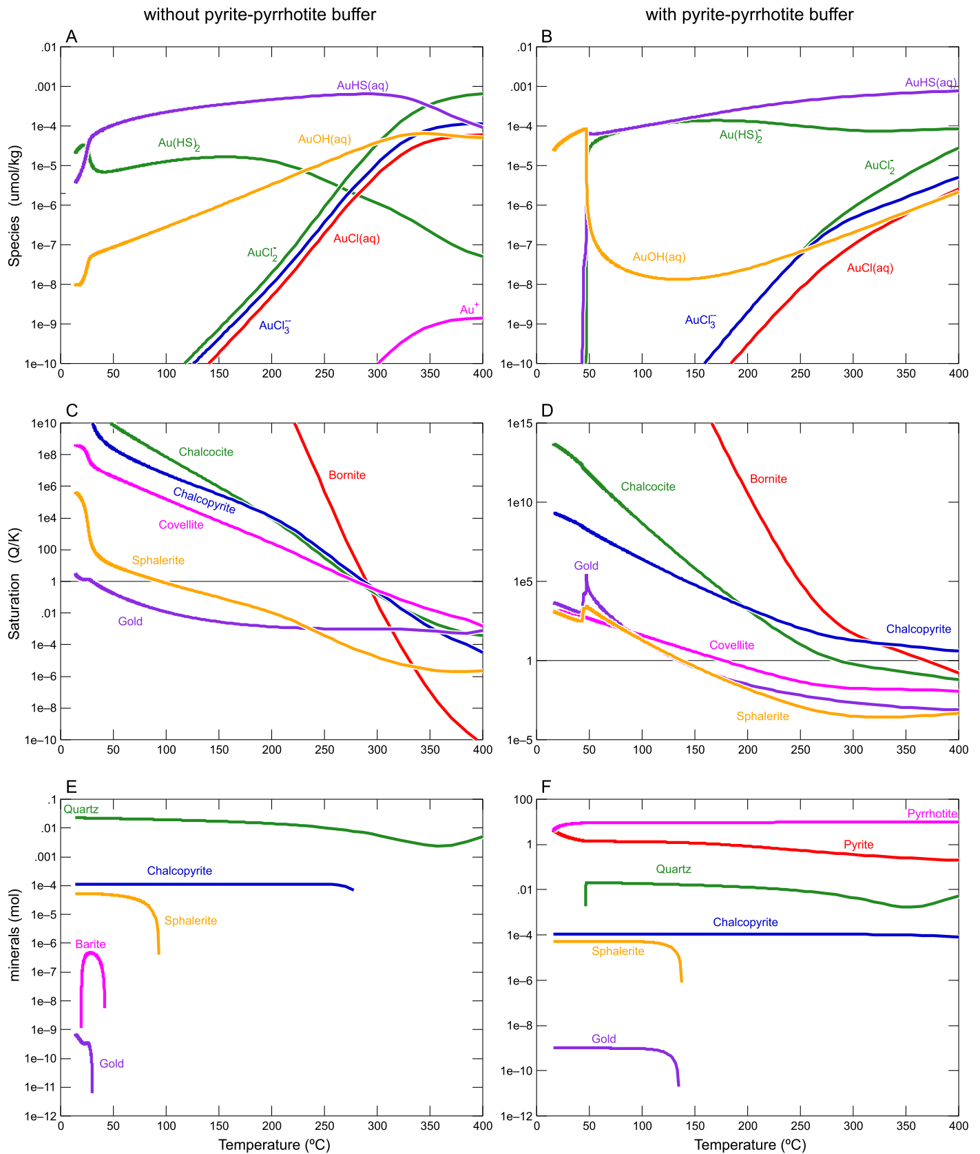
Figure 5. Results of thermodynamic calculations, as in Figure 4, except cooling is achieved by mixing with ambient seawater.
