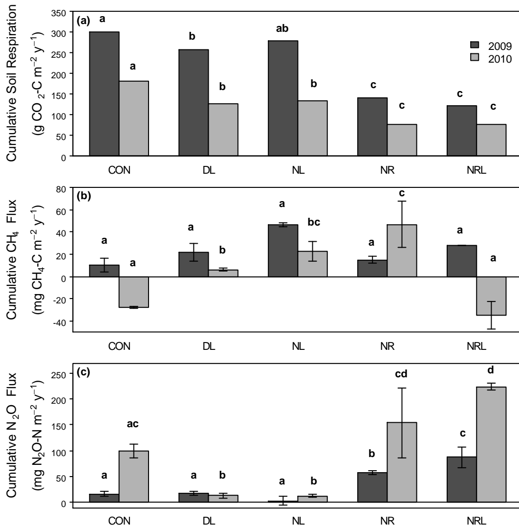
Figure 5.3 – Cumulative soil-to-atmosphere fluxes for 2009 (dark grey bars) and 2010 (light grey bars) of a ) Soil respiration, b ) Methane (CH 4 ) and c ) Nitrous oxide (N 2 O). Values for soil respiration are cumulative modelled fluxes. Values for CH 4 and N 2 O are extrapolated from the mean cumulative sums from each plot and bars represent standard error values. Significant differences (ANOVA and pair-wise post-hoc comparisons, p < 0.05, at 1, 23 df ) between treatments in each year are indicated by different letters.
