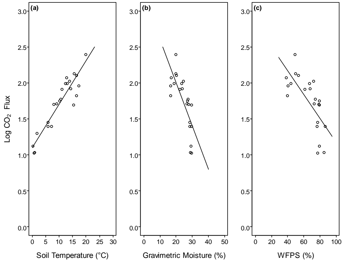
Figure 2.4 - Correlations between logged CO 2 flux and a ) Soil temperature (0-7 cm depth), b ) gravimetric moisture (0-15 cm, depth) and c ) Water-filled pore space (WFPS) (0-15 cm, depth). Values are mean monthly values (n=5).
