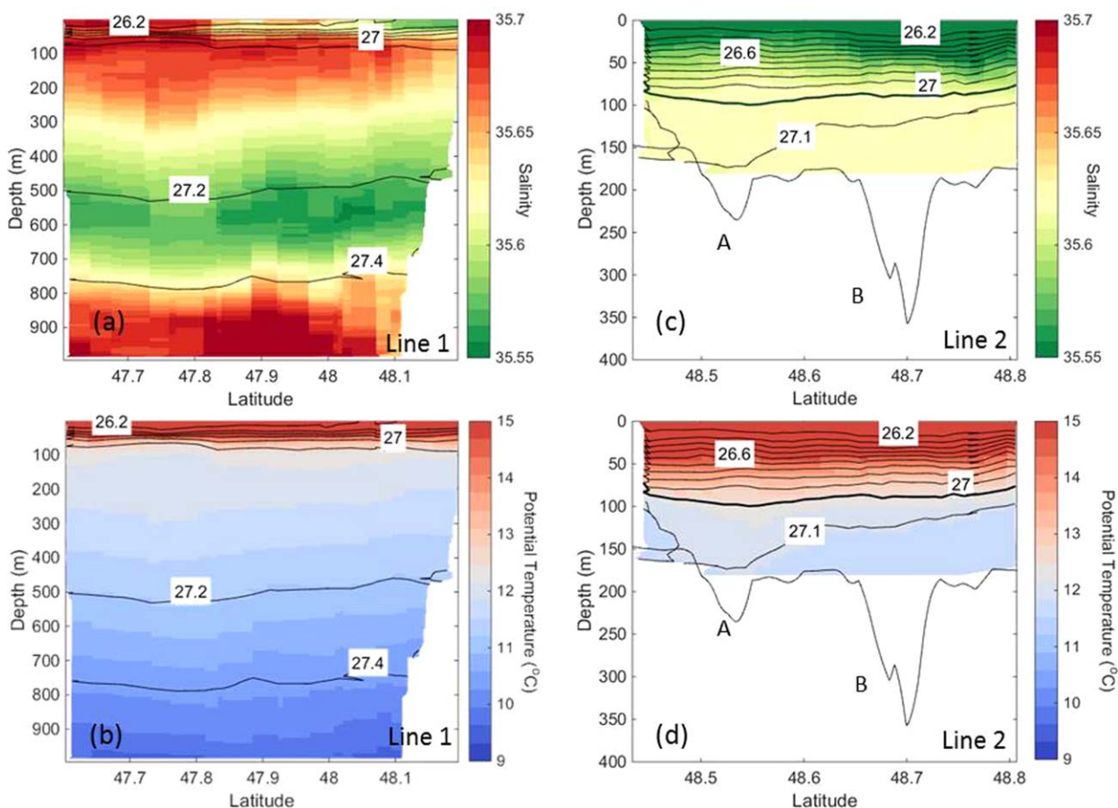
Figure 8. Time mean transects between 5 August and 15 August, during which time the slope current was poleward. The transects are from (a, b) transect 1 and glider 330 and (c, d) transect 2 and glider 194. (a, c) Salinity, (b, d) temperature. (c–e) The black contours indicate the density and the lowest line on each plot is the bathymetry at the shelf-break, with the canyons A and B (Figure 1) labeled.
