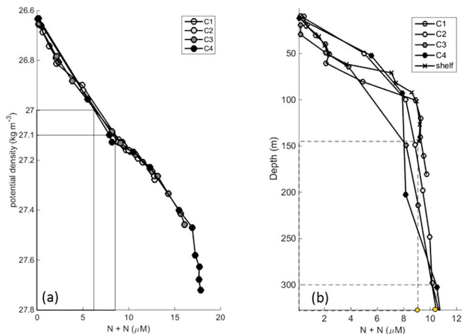
Figure 10. (a) Potential density profiles of Nitrate + Nitrite at 4 points along the Petite Sole canyon (C1:C4, where C1 is on the shelf and C4 at the mouth of the canyon). The solid lines indicate the background shelf density ( 27 \text{ kg m}^{-3} ) and the density within the salinity cores ( 27.1 \text{ kg m}^{-3} ), with N+N values recorded from the mid point of the 4 profiles. (b) Nitrate + Nitrite at the same 4 points in the canyon and on the shelf, shelfward of the canyon (shelf). The dashed line indicate the maximum upwelling depth and the depth of the center of the salinity cores, the yellow dots show where the C4 and shelf profiles intersect the y axis.
