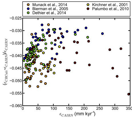
Figure 10. Differences between the denudation rate calculated by CAIRN ( \epsilon_{\text{CAIRN}} ) and the denudation rate calculated with CRONUScalc ( \epsilon_{\text{CRCalc}} ) as a function of CAIRN denudation rate for selected studies.
