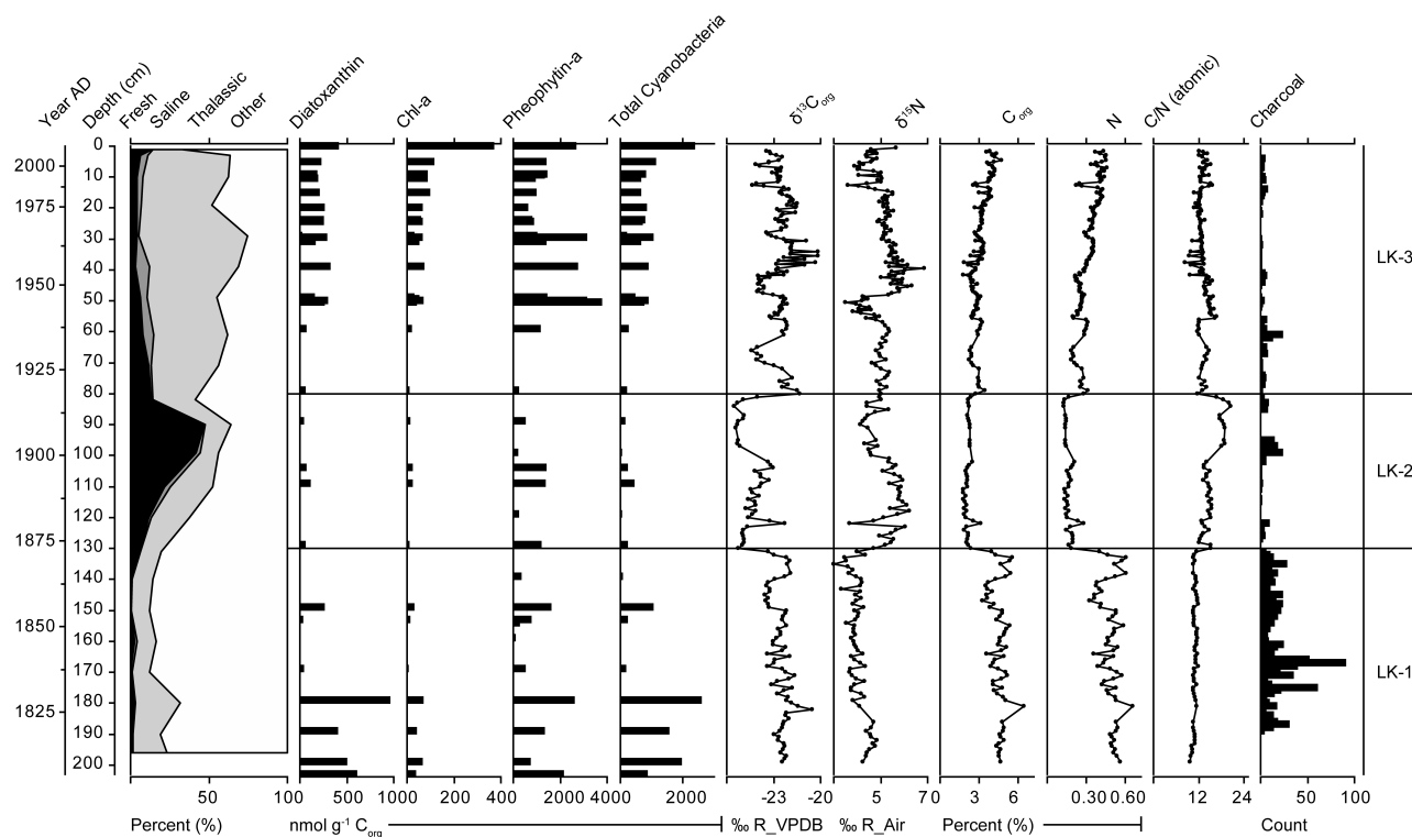
Figure 3. Depth profiles for the site Lake King north of diatom salinity indicator species (See Fig. 4 for classification of species) and geochemical proxies including pigments chlorophyll a (Chl a ), pheophytin a and total cyanobacteria (the sum of the pigments, zeaxanthin, canthaxanthin and echinenone) normalized to sediment organic-carbon content. Sediment organic carbon and nitrogen isotope ratios ( \delta^{13}\text{C} and \delta^{15}\text{N} respectively). Sediment organic carbon and total nitrogen content (percentage of sediment mass) and their ratio ( \text{C}_{\text{org}} , N, C/N respectively). Charcoal content of the sediment expressed in particles per millilitre. The zones LK-1 to LK-3 are three regions of the profile corresponding to inflections in DCA axis 1 (See Fig. 4) and also abrupt changes in the carbon and nitrogen isotope and concentration proxies.
