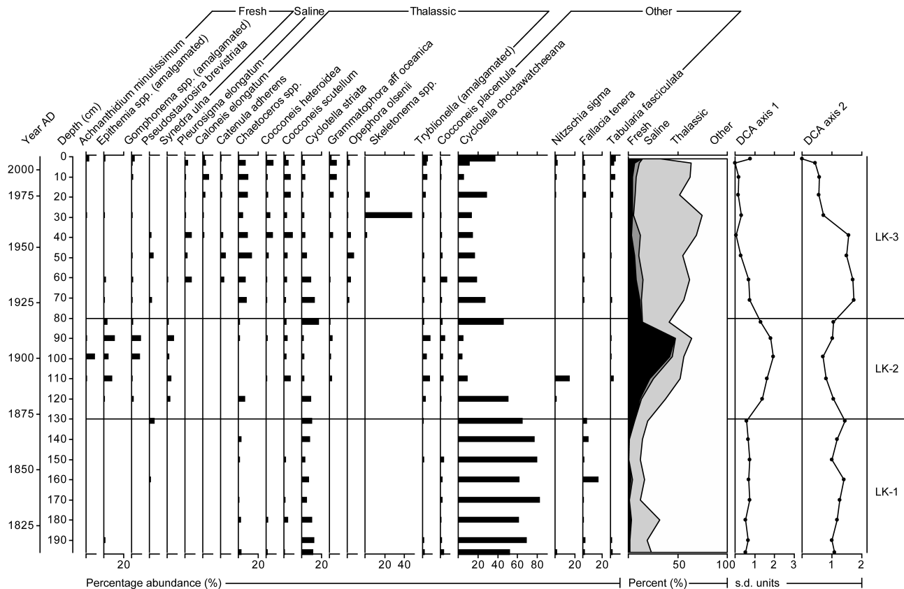
Figure 4. Profiles of diatom species abundance (percentage of total species count) grouped based on water salinity (fresh, saline, thalassic and other). Fresh indicates diatoms found at salinities <5, saline indicates species expected to grow at high salinity within estuaries, and thalassic species are expected to be found exclusively in the coastal ocean. Other refers to species typical of intermediate salinity within estuaries and lagoons. Detrended correspondence analysis (DCA) axes 1 and 2 are also shown with depth.
