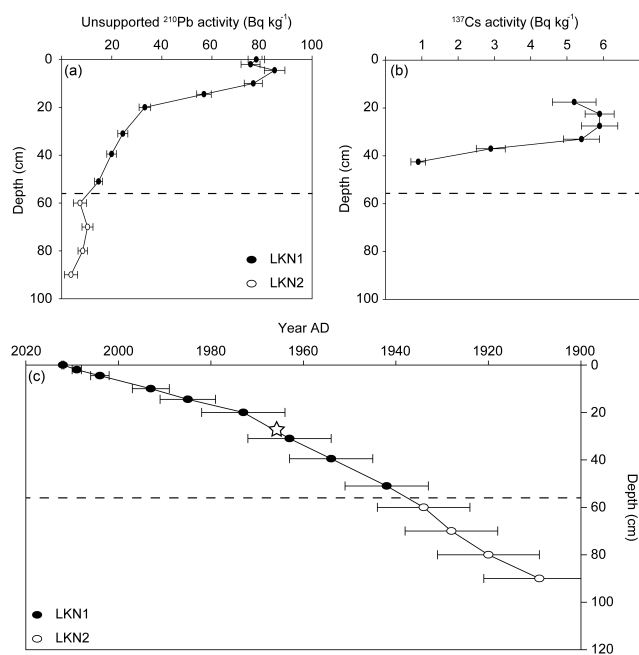
Figure 2. Unsupported ^{210}\text{Pb} activities ( \text{Bq kg}^{-1} sed) versus depth (a), ^{137}\text{Cs} activities ( \text{Bq kg}^{-1} sed) versus depth (b) and the age depth model based on unsupported ^{210}\text{Pb} values using the CIC (constant initial concentration) model (c). The star in (c) refers to the depth of the ^{137}\text{Cs} peak activity. LKN1 and LKN2 refer to the two different cores sampled (see methods) and the horizontal dashed line demarcates the transition from core LKN1 to LKN 2.
