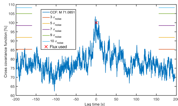
Figure A9. Averaged absolute CCF of mass 71.0851 (could not be identified), which fulfilled the 7\sigma_{\text{noise}} criteria.
