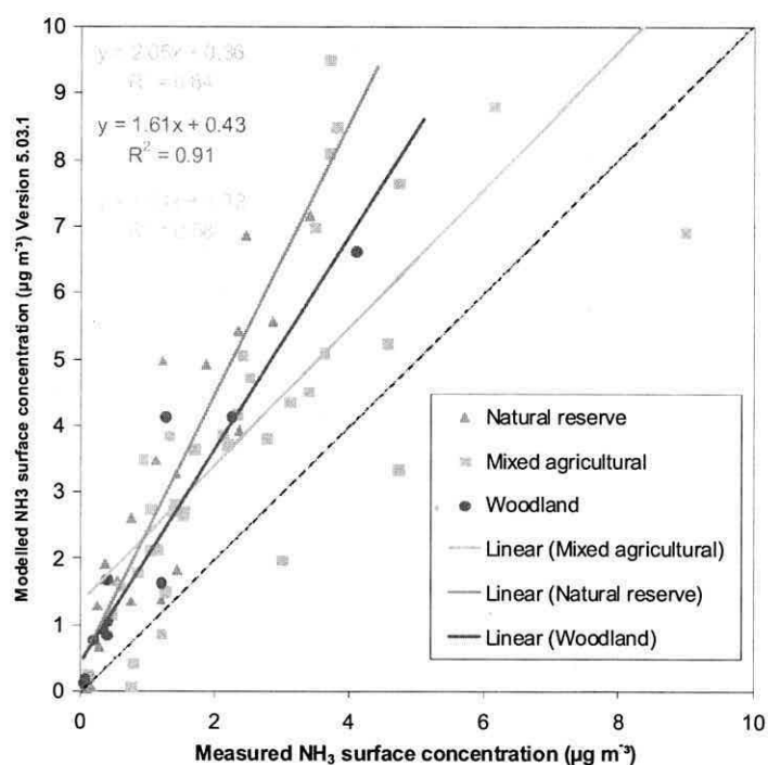
Figure 8.2 FRAME \text{NH}_3 predictions versus UK National ammonia monitoring network. Units are \mu\text{g m}^{-3} .
