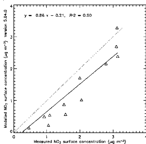
Fig. 4(d) Modelled \text{NO}_3^- concentration correlation with measurements
