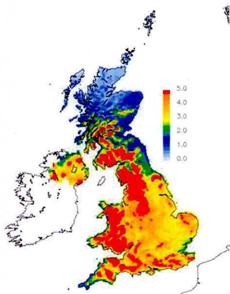
Fig. 3.3(a) FRAME 2002 \text{NH}_x wet deposition [ \text{kg N ha}^{-1} \text{yr}^{-1} ]
