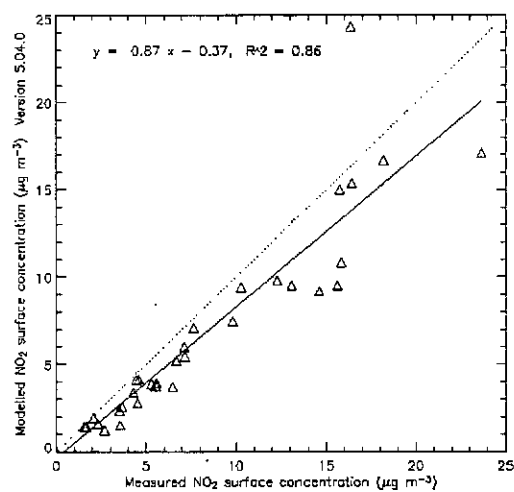
Fig. 4(c) Modelled \text{NO}_2 concentration correlation with measurements
