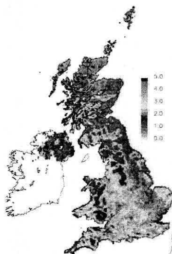
Figure 11.1(b) FRAME 2002 SO x wet deposition (kg S ha -1 yr -1 )
