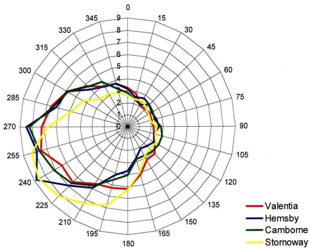
Figure 5.3: Average wind frequency rose for different stations calculated from 1991-2000 radiosonde data. Radial units are percent per 15° direction band
