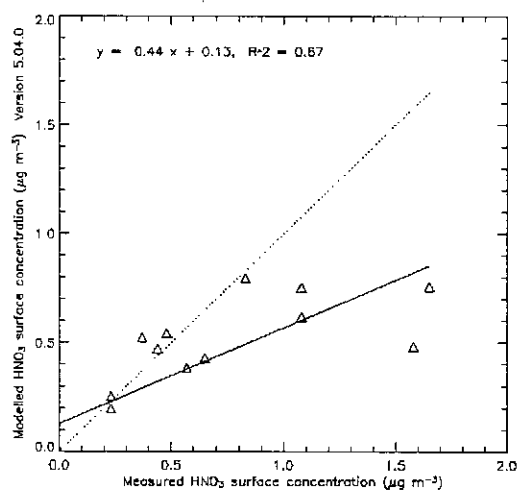
Fig. 4(g) Modelled \text{HNO}_3 concentration correlation with measurements
