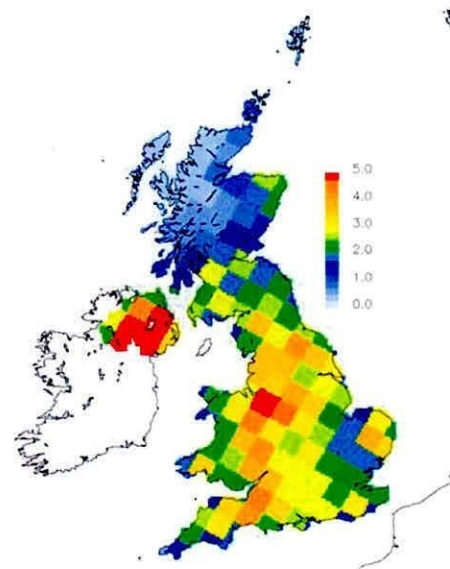
Fig. 3.3(f) EMEP 2002 \text{NH}_x dry deposition [ \text{kg N ha}^{-1} \text{yr}^{-1} ]
