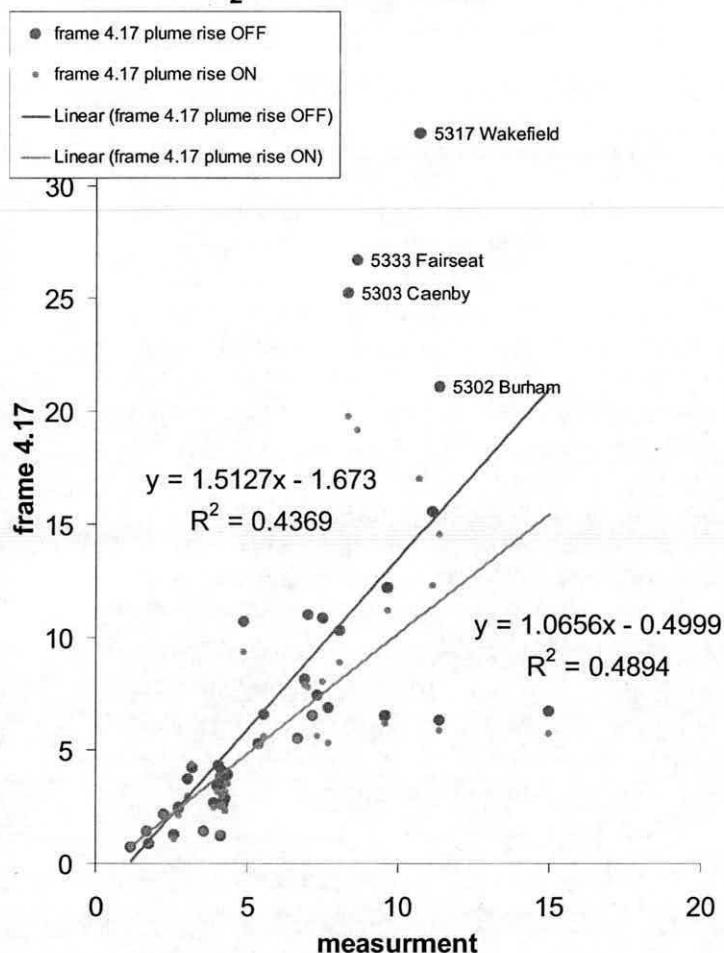
Figure 7.1(a) Correlation of modelled SO 2 concentrations ( \mu\text{g m}^{-3} ) with measurements for the year 1999 with (i) no plume rise parameterisation and (ii) plume rise parameterisation included
