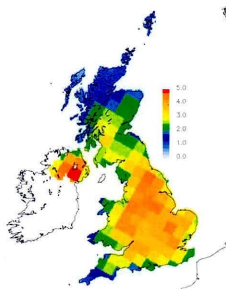
Fig. 3.3(c) EMEP 2002 \text{NH}_x wet deposition [ \text{kg N ha}^{-1} \text{yr}^{-1} ]
