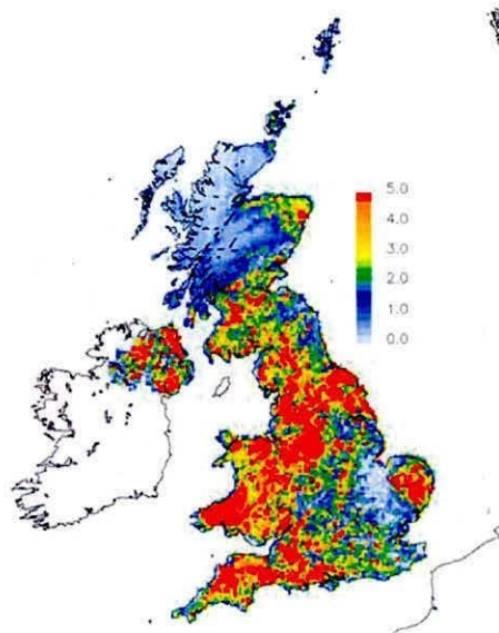
Fig. 3.3(e) CBED 2001-03 \text{NH}_x dry deposition [ \text{kg N ha}^{-1} \text{yr}^{-1} ]
