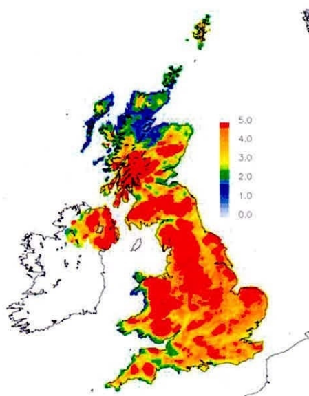
Fig. 3.3(b) CBED 2001-3 \text{NH}_x wet deposition [ \text{kg N ha}^{-1} \text{yr}^{-1} ]
