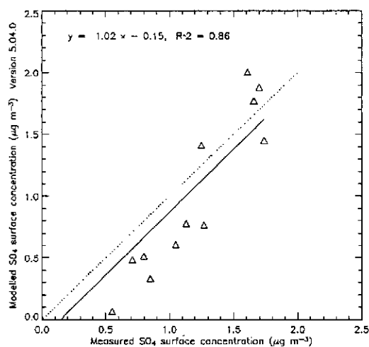
Fig. 4(b) Modelled \text{SO}_4^{2-} concentration correlation with measurements
