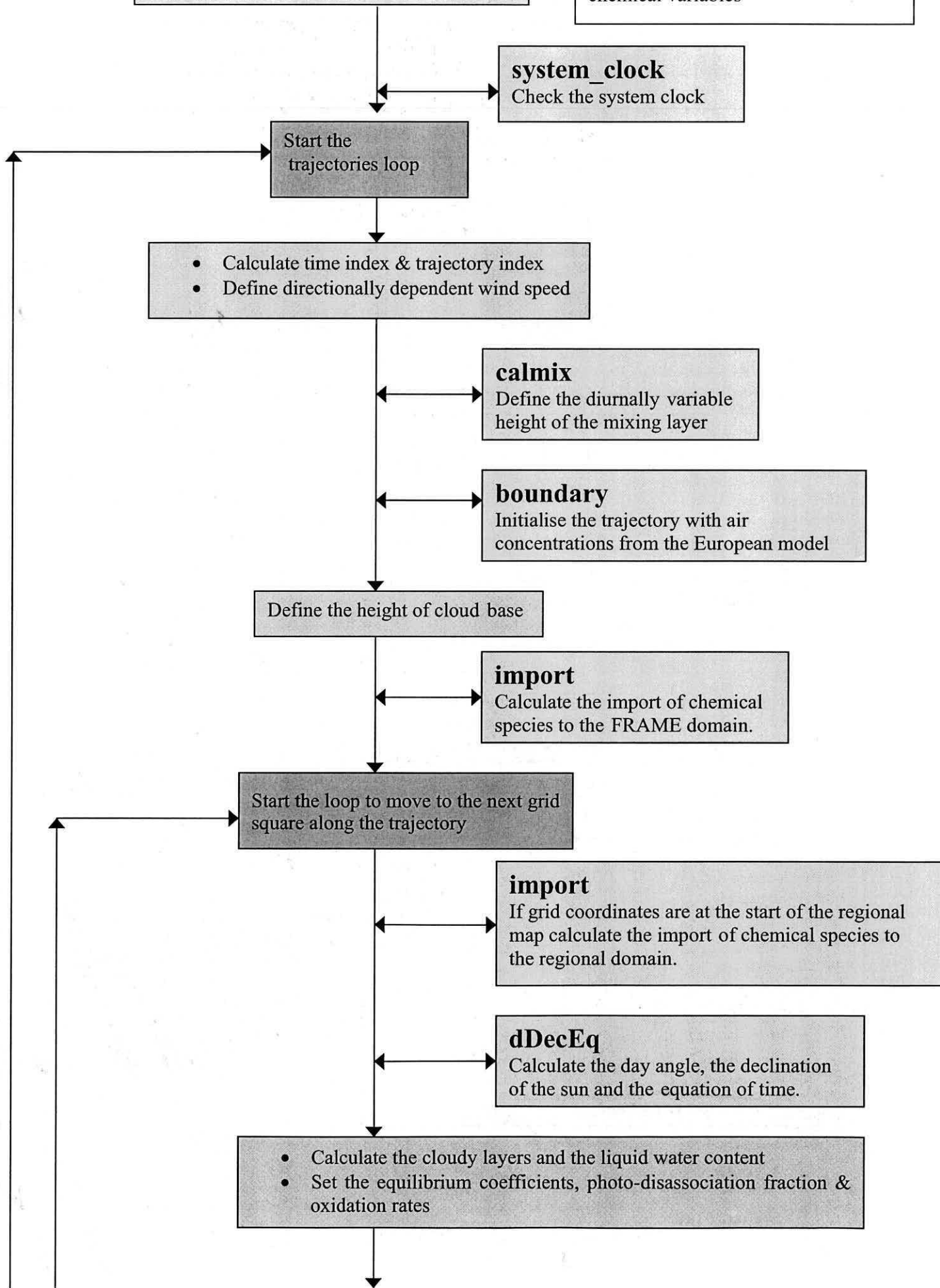
Figure 3 Flow chart illustrating the sequence of routines used to advect trajectories and update physical and chemical variables
