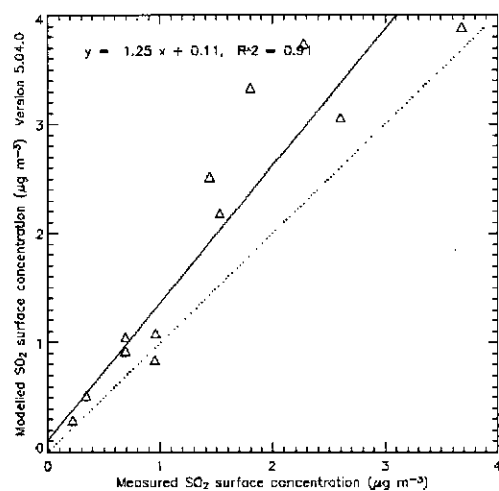
Fig. 4(a) Modelled \text{SO}_2 concentration correlation with measurements
