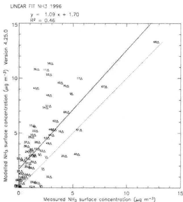
Figure 7.2(a) Correlation of modelled \text{NH}_3 concentrations ( \mu\text{g m}^{-3} ) with measurements for the year 1996 with all emissions input to the surface layer
