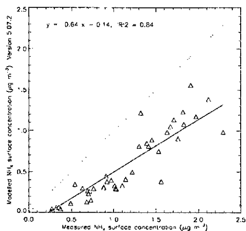
Fig. 4(f) Modelled \text{NH}_4^+ concentration correlation with measurements
