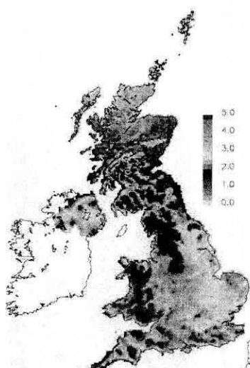
Figure 11.1(f) FRAME 2002 NH x wet deposition (kg N ha -1 yr -1 )
