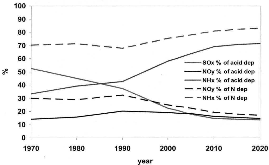
Figure 12.4(b) The relative contributions to acidic and nitrogen deposition to forest of \text{SO}_x , \text{NO}_y and \text{NH}_x in the UK during the period 1970 to 2020
