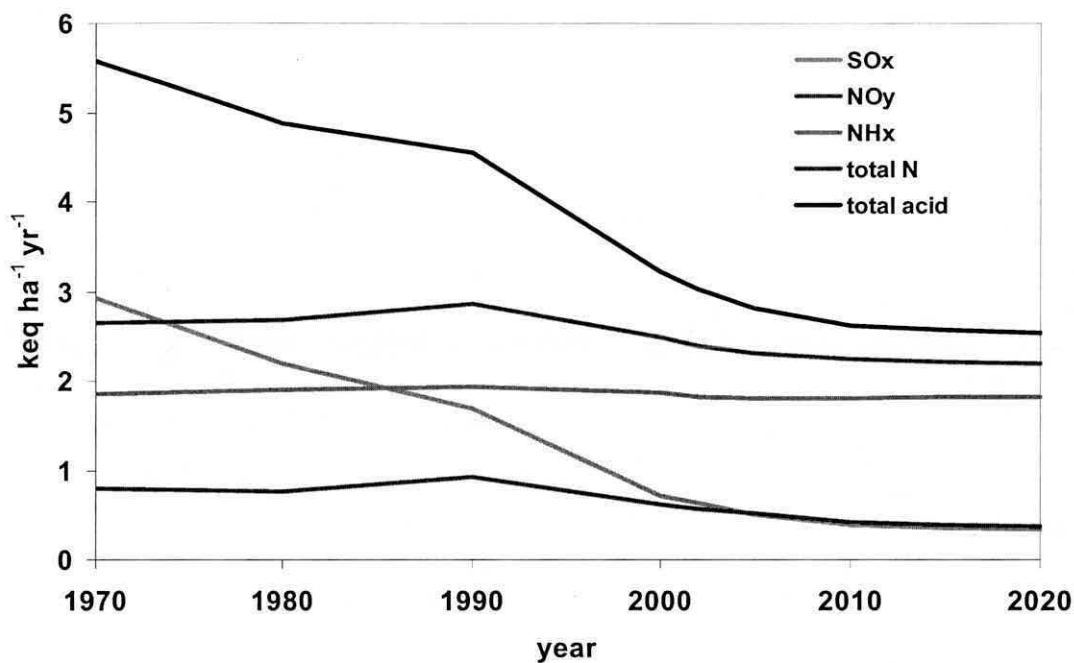
Figure 12.4(a) Average deposition to forest in the UK of \text{SO}_x , \text{NO}_y and \text{NH}_x during the period 1970 to 2020
