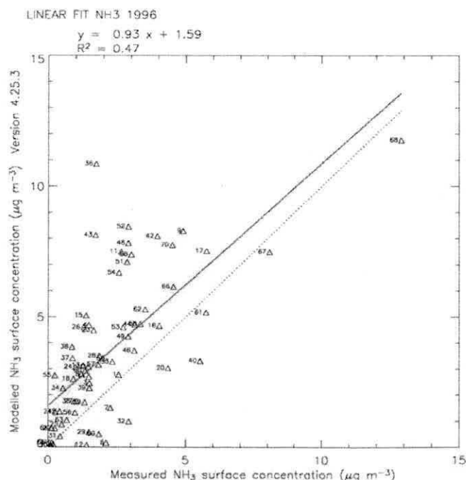
Figure 7.2(b) Correlation of modelled \text{NH}_3 concentrations ( \mu\text{g m}^{-3} ) with measurements for the year 1996 with sector specific emissions height
