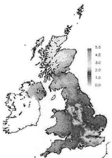
Figure 11.2(e) FRAME 2020 NO y dry deposition (kg N ha -1 yr -1 )
