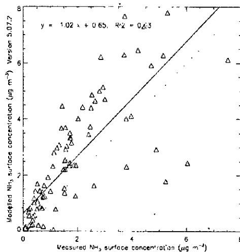
Fig. 4(e) Modelled \text{NH}_3 concentration correlation with measurements
