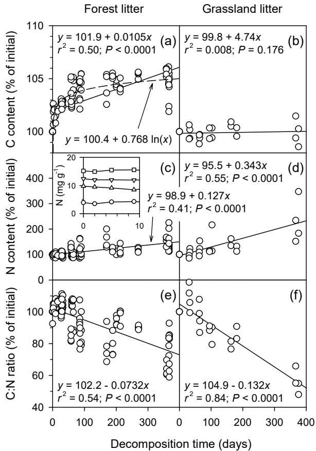
Figure 4. Total C, N and C:N ratio relative to the initial level at the beginning of the decomposition period. The data correspond to reciprocal litter transplantation experiments with leaf litter from forest sites: Pinus sylvestris (Hyytiälä, Finland), Pinus sylvestris (Männikjärve, Estonia), Fagus sylvatica (Sorø, Denmark), and Pseudotsuga menziesii (Speulderbos, Netherlands); and grassland sites: Lolium perenne (Easter Bush, UK) and Festuca pseudovina (Bugac, Hungary). Data points ( N = 112 for tree litter and N = 24 for grass litter) are the average value of three litter bags. In (a), the dashed line represents the best logarithmic fit to the data. The inset in (c) represents the N content in leaf litter during the first 10 days of decomposition. Symbols stand for P. sylvestris from Hyytiälä (○) and Männikjärve (▽), F. sylvatica (Δ), and P. menziesii (□).
