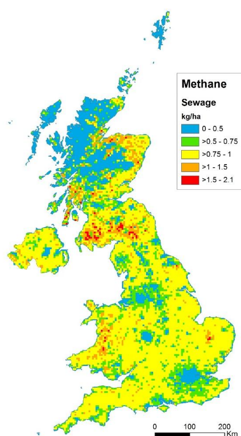
Figure 16. Methane emissions sewage spreading
