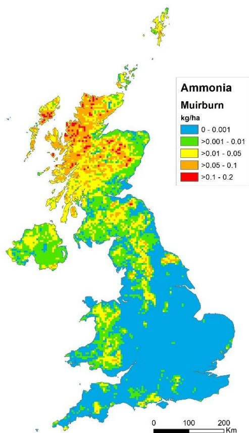
Figure 3. Ammonia emissions from biomass burning
