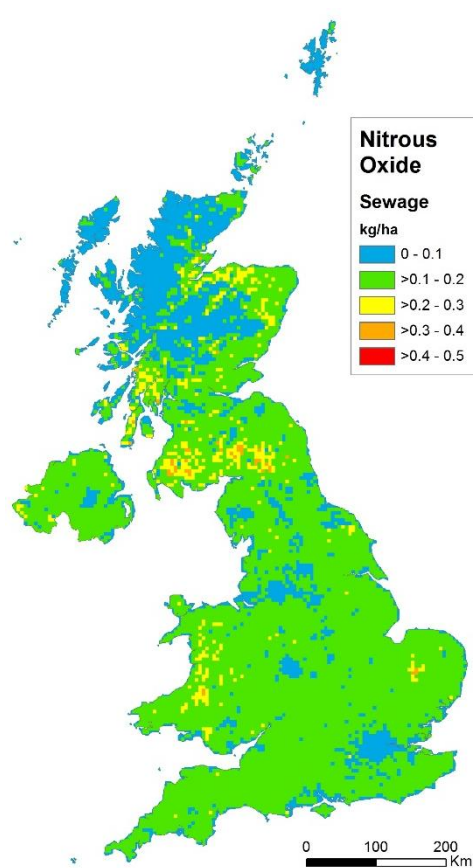
Figure 18. Nitrous oxide emissions sewage spreading
