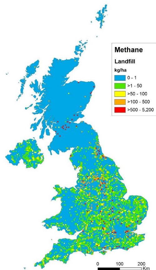
Figure 15. Methane emissions from landfill
