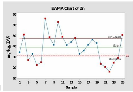
Fig. 3 EWMA charts of Cd, Cu, Pb and Zn distribution in moss samples (Centre Line–Kosovo median value; dashed line–European median value; LCL - lower control limit, LCL=median-2SDEV; UCL – upper control limit, UCL=median+2SDEV)
