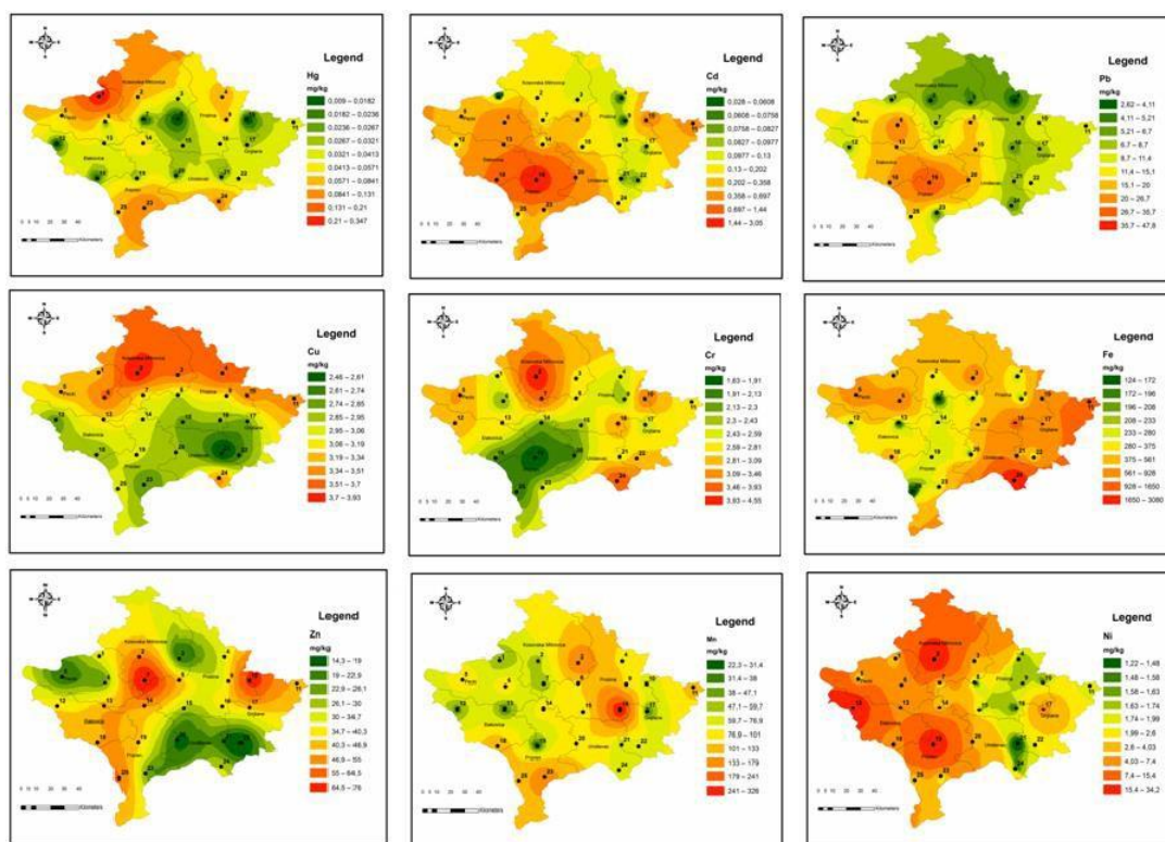
Fig. 1 The GIS maps of trace metal atmospheric deposition in Kosovo
