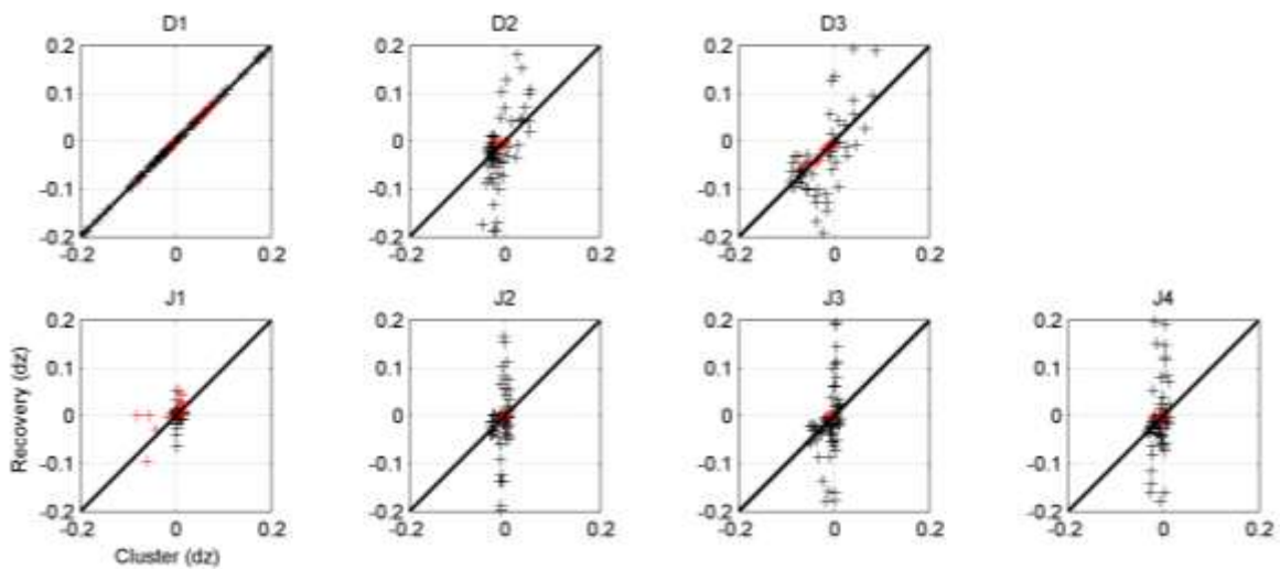
Figure 9 Comparison of bed level change ( dz = z_{final} - z_{initial} , z :bed level) at each point along the profile within each storm event during the cluster and recovery applications, negative indicates erosion and positive incates accretion. Black '+' indicates below and red '+' indicates above the threshold dune erosion elevel (3.9 m ODN). For the clarity, -0.2 to 0.2 range is shown.
