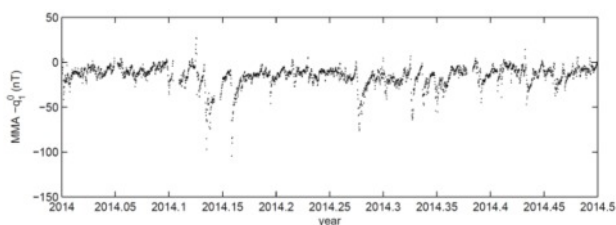
North-South component of the magnetospheric field derived from Swarm data over the first six months of 2014
