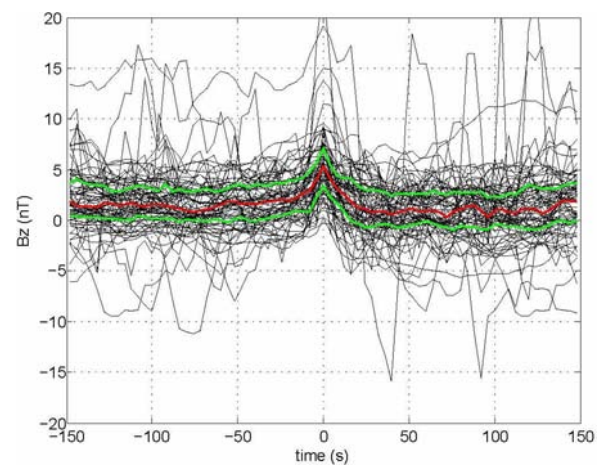
Signature of tail-ward-propagating dipolarisation fronts in the Z-component of the magnetic field in Cluster spacecraft data. Red (green) is the mean (mean +/- 1 standard deviation) level from a number of superposed events.(Nina Kahr)
