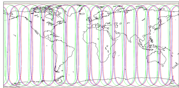
Orbit tracks of Swarm A (red), B (green), and C (blue) over one day (21 September, 2014)
