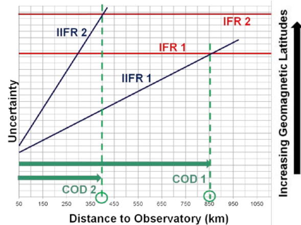
Schematic to demonstrate the improvement in uncertainty using IIFR over IFR and how this drops off with distance from the drilling location. Two example geomagnetic latitudes (1=lower and 2=higher latitude) are show. The COD is reached when IIFR (blue) no longer reduces the uncertainty compared to IFR (red).
