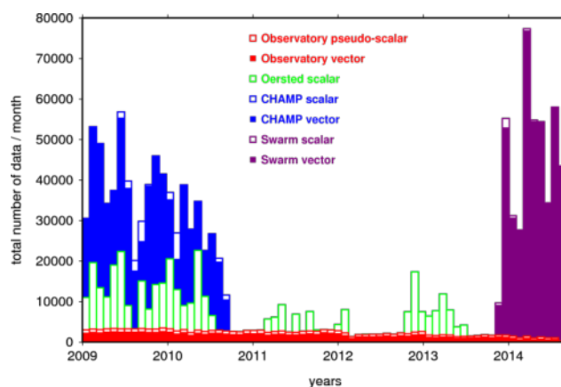
Total number of selected (geomagnetically quiet) data per month for IGRF-12 candidate models from each measurement platform
