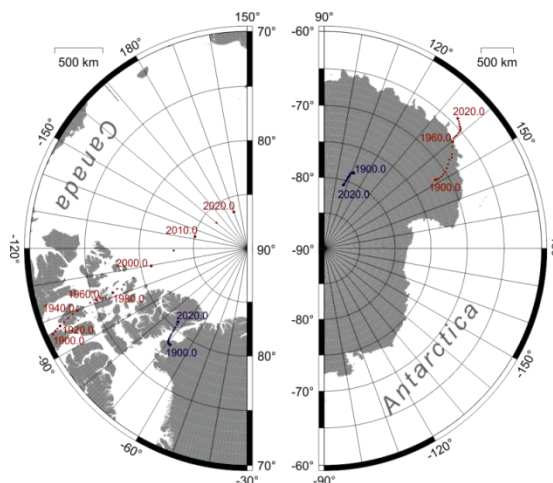
Geomagnetic (blue) and dip (red) poles from the IGRF-12 field model
