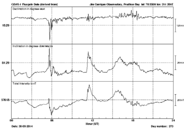
Magnetogram showing typical variations in declination (top), inclination or dip (middle) and total field intensity (bottom) at JCO, Alaska. This day is not classed as an 'International Disturbed Day' yet declination changes by >4^\circ
