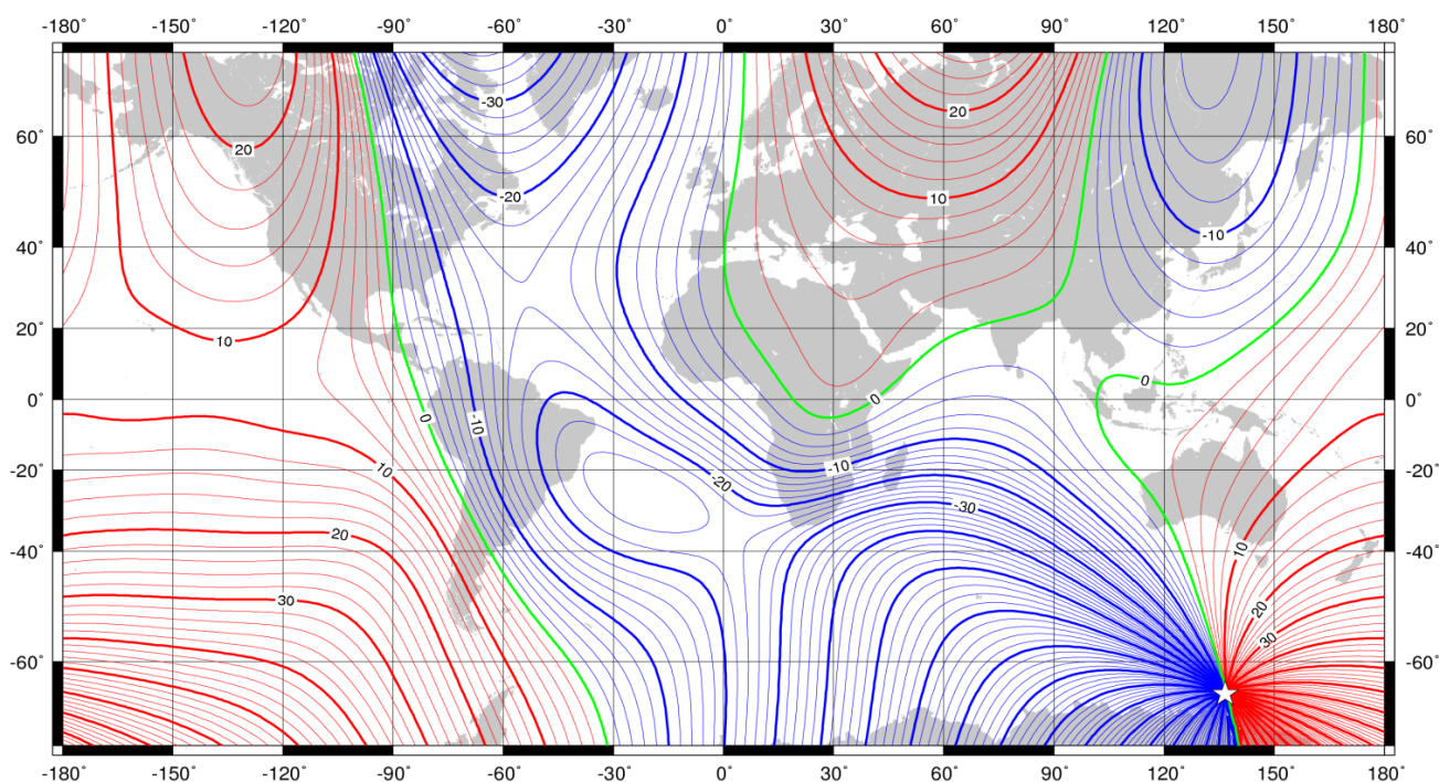
Declination (magnetic variation) at 2015.0 from the World Magnetic Model (WMM2015). Red - positive (east), blue - negative (west), green - zero (agonic line). Contour interval is 2^\circ , white star is location of a magnetic pole and projection is Mercator. This is an example of an isogonic chart. Credit: British Geological Survey (Natural Environment Research Council).
