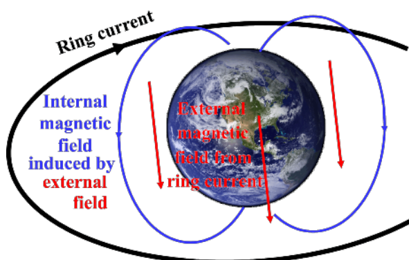
Simplified diagram of the Earth's ring current (black) and the magnetic fields it produces: external (red) and induced internal (blue)
