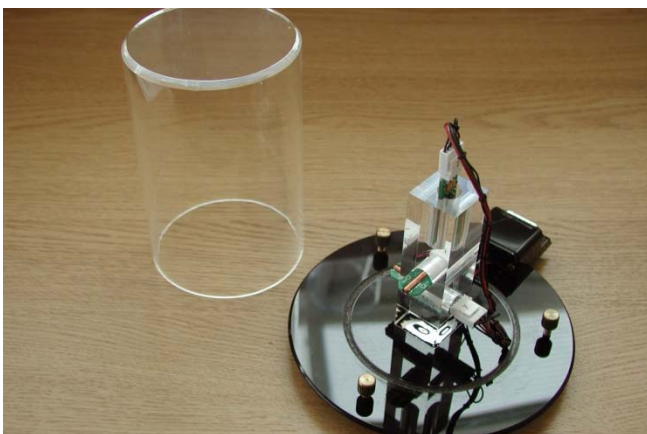
Prototype 3-Component Fluxgate sensor for the School Magnetometer
