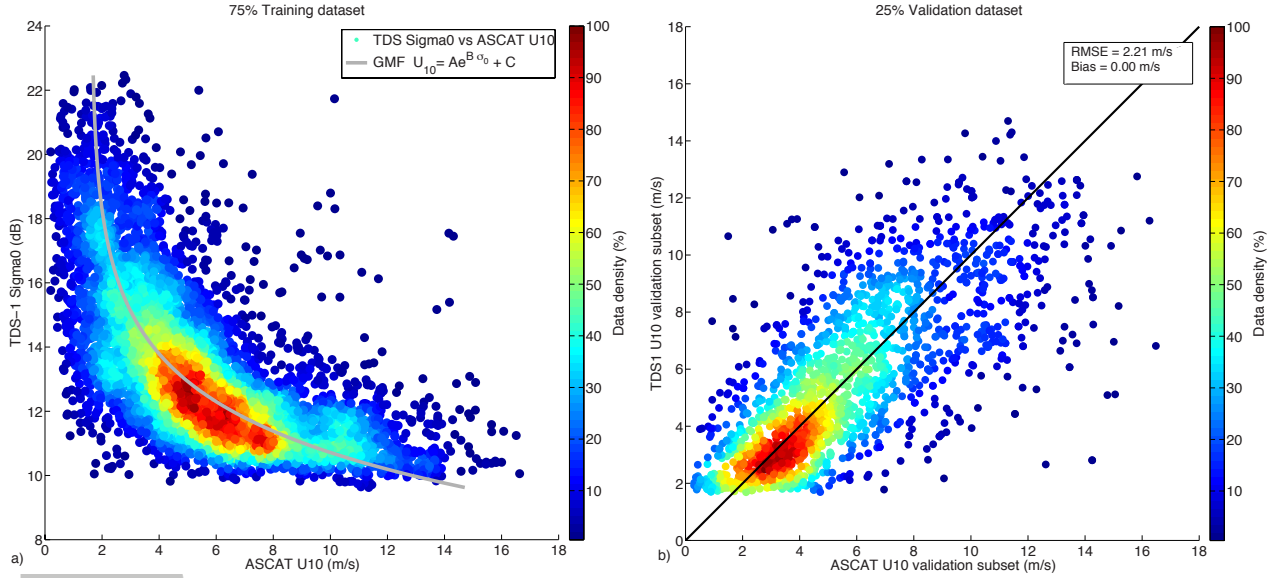
Figure 4. a) TDS-1 ReSI uAGC mode Sigma0 versus collocated ASCAT wind speed for \text{SNR} \geq 3\text{dB} for the Training dataset, showing (in grey) the preliminary GMF of the form U_{10} = Ae^{B\sigma_0} + C with values of A, B and C equal to 676.0, 0.4097 and 1.622 respectively; b) TDS-1 ReSI wind speed retrieved with the BRE algorithm versus collocated ASCAT winds for the Validation dataset. This example validation dataset yields bias and RMSE values of 0.004 m/s and 2.213 m/s respectively and is statistically representative of the overall BRE retrieval performance.
