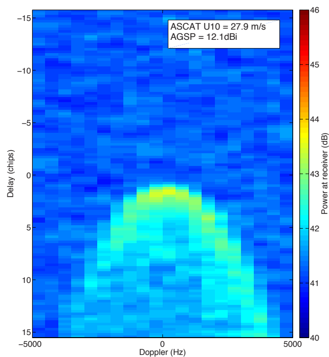
Figure 3. TDS-1 ReSI onboard-processed 1 Hz delay Doppler Map obtained for a wind speed of 27.9 m/s (according to collocated ASCAT data) in the Atlantic sector of the Southern Ocean on 31 October 2014
