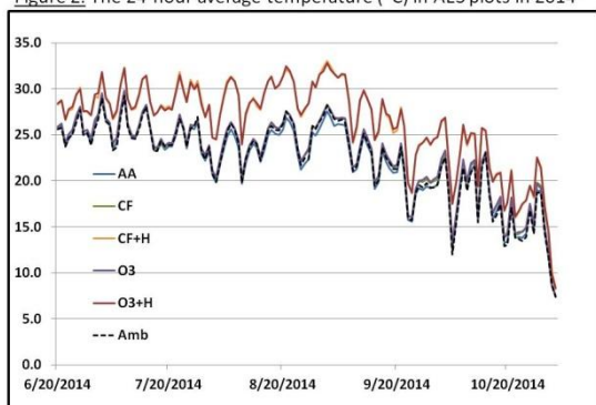
Figure 2. The 24-hour average temperature (°C) in AES plots in 2014
