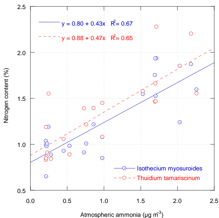
Figure 1. Nitrogen content (%) in two moss species ( Isoetium myosuroides and Thuidium tamariscinum ) against atmospheric ammonia ( \text{NH}_3 ) concentrations ( \mu\text{g m}^{-3} ).
