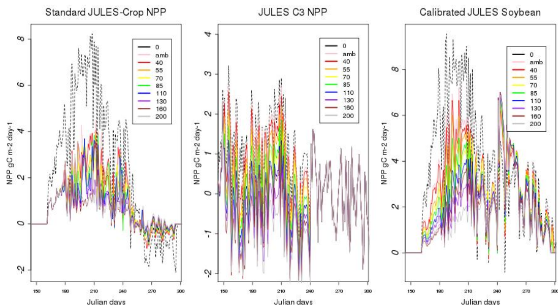
Figure 1. Simulations of the Net Primary Productivity of soybean of different target ozone using: (from left to right) standard JULES-Crop, standard JULES with C3 grass instead of soybean, calibrated and tuned JULES-Crop parameters
