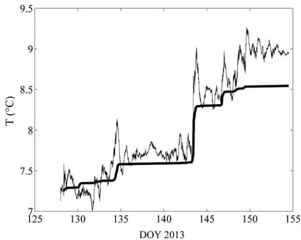
Fig. 14. Heat flux and water column heat content. The fine line shows the average temperature of the water column below the ADCP which was measuring dissipation during deployment 3. The thick line represents the temperature rise resulting from the pycnocline heat flux based on the observed dissipation.
