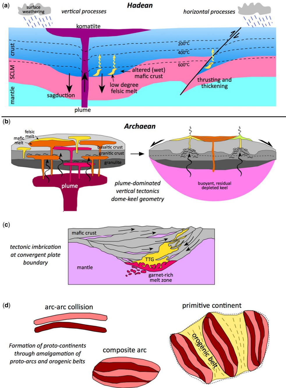
Fig. 6. (a) Model of Hadean crust formation comprising mafic protocrust and small amounts of low-degree felsic melts (modified from Nebel et al. 2014). (b) Plume-dominated Archaean crust formation that may have dominated the early Archaean, with eruption and intrusion of mantle-derived mafic magmas and intracrustal reworking to form felsic magmas. Vertical tectonics is dominant, and leads to a dome and keel structure (modified from Van Kranendonk et al. 2011). (c) A model of crust formation in 'proto-arcs' that may have arisen in the early Archaean, featuring imbrication of oceanic crust rather than deep subduction, and production of felsic magmas from deep melting of mafic crust (after Nutman et al. 2007). (d) The amalgamation of 'proto-arcs' into primitive continents through their accretion and collision (after Santosh et al. 2009).
