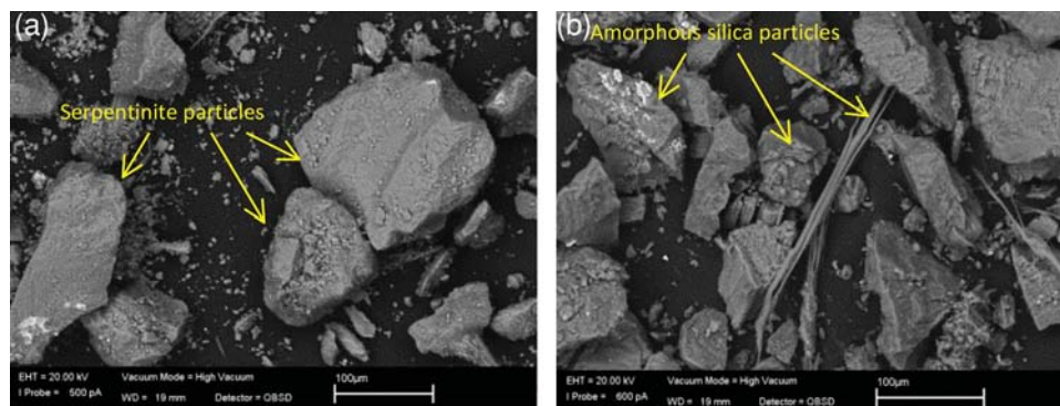
Figure 9. BSE photomicrographs of serpentinite rock powder before (a) and after (b) acid leaching of Mg ions. The Mg-rich silicate is transformed into silica-rich particles retaining the morphology of the original material.
