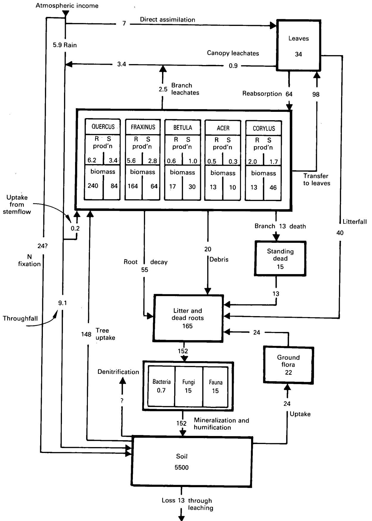
Figure 1. The nitrogen cycle of the mixed deciduous woodland in Meathop Wood, UK; nitrogen contents in kg ha -1 and annual net transfers in kg ha -1 yr -1
