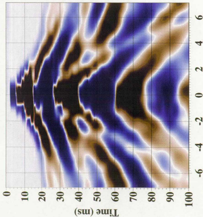
Acoustic moveout
