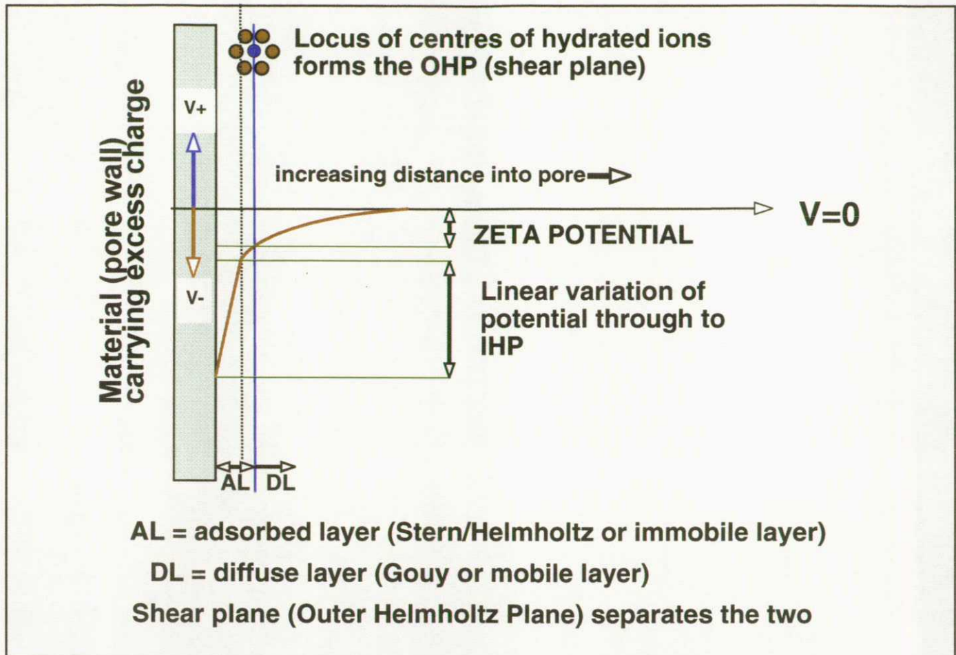
Figure 4.2. Schematic of the potential distribution across the electrical double layer.
