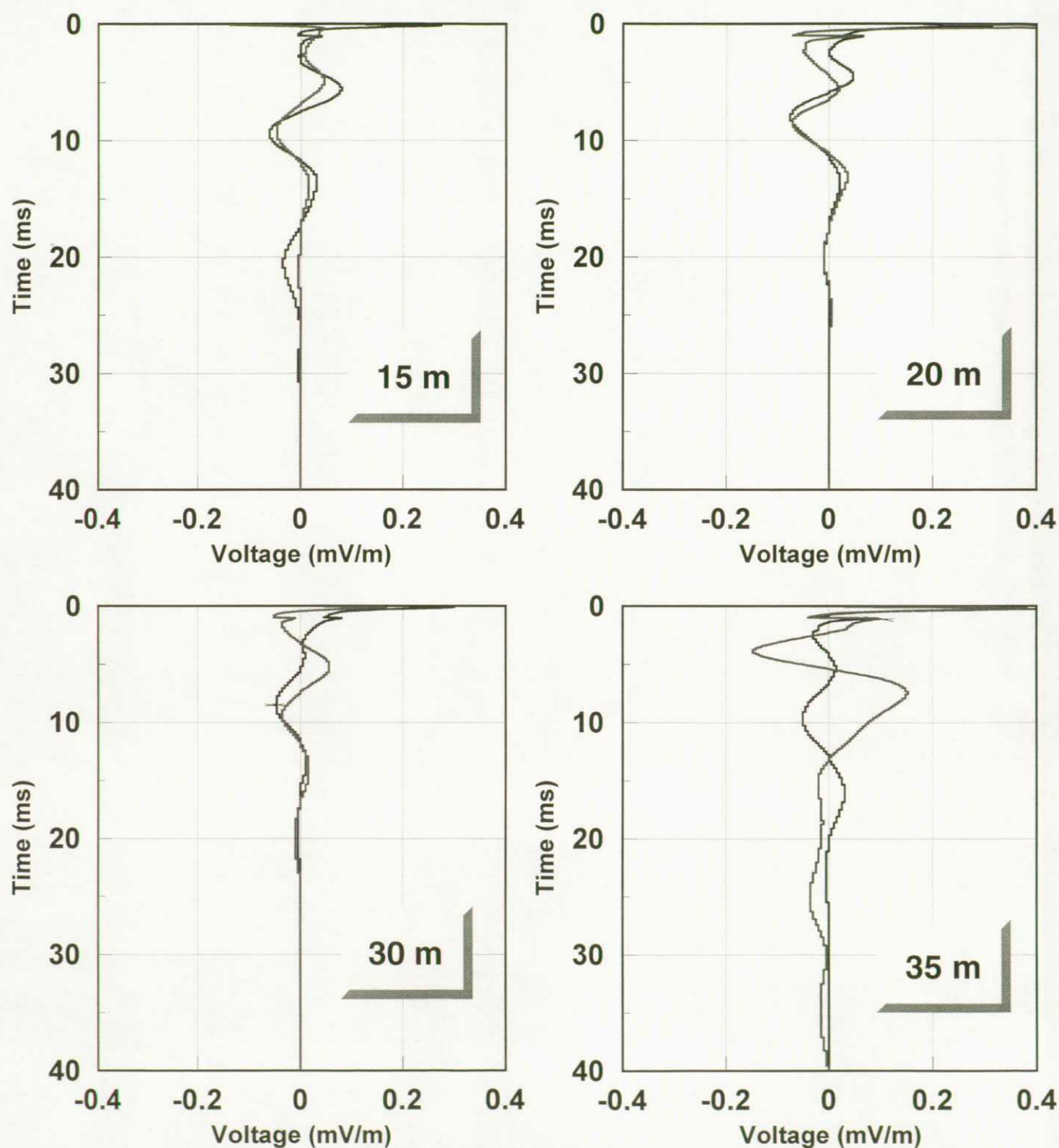
Figure 5.7 2-channel EK-sounding curves in Voltage/time. Two sets of adjacent (5m) soundings. Typical Clay response (Note voltage scale).
