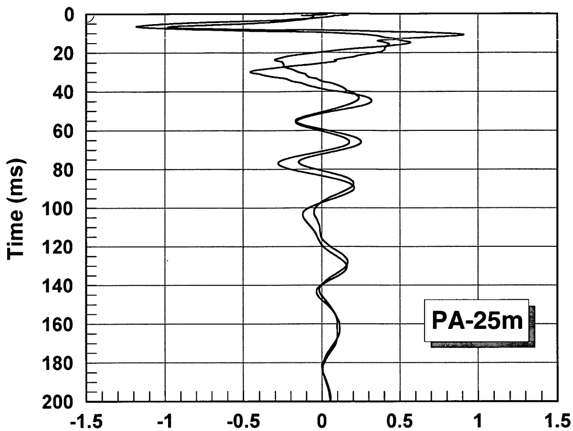
Figure 6.12 EK sounding at 25 m along profile PA. Postbridge survey, Dartmoor granite
