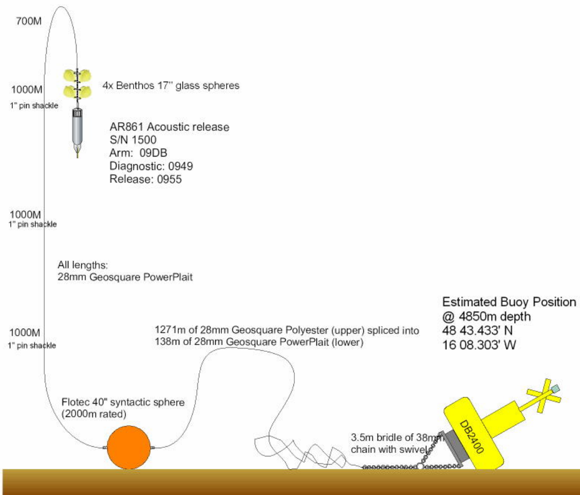
Figure 2: Diagram showing the layout of the OSMOSIS PAP site mooring array as estimated from the triangulation process on D381.
