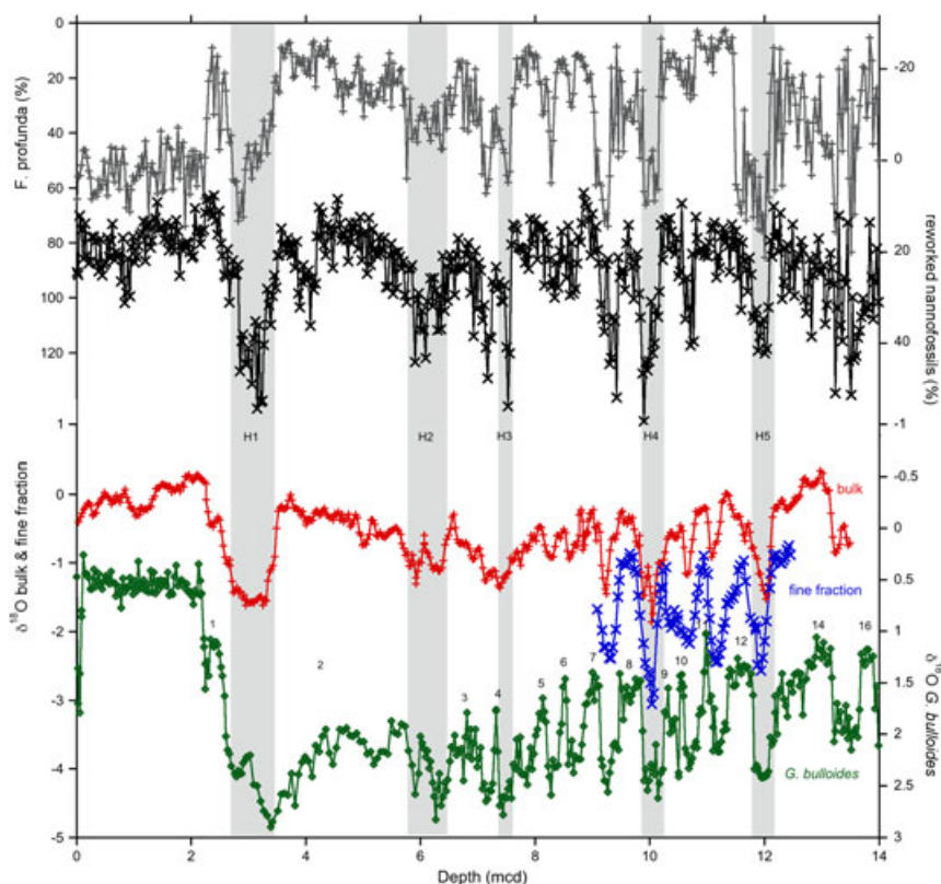
Figure 9. \delta^{18}\text{O} of G. bulloides (green), fine-fraction \delta^{18}\text{O} (<63m; blue), bulk \delta^{18}\text{O} (red), percent reworked nannofossil taxa (black), and percent Florisphaera profunda (gray) [Incarbona et al. , 2010] in Core MD01-2444. Heinrich stadials are marked by high planktic \delta^{18}\text{O} , low bulk \delta^{18}\text{O} , and increased reworking and abundances of F. profunda .
