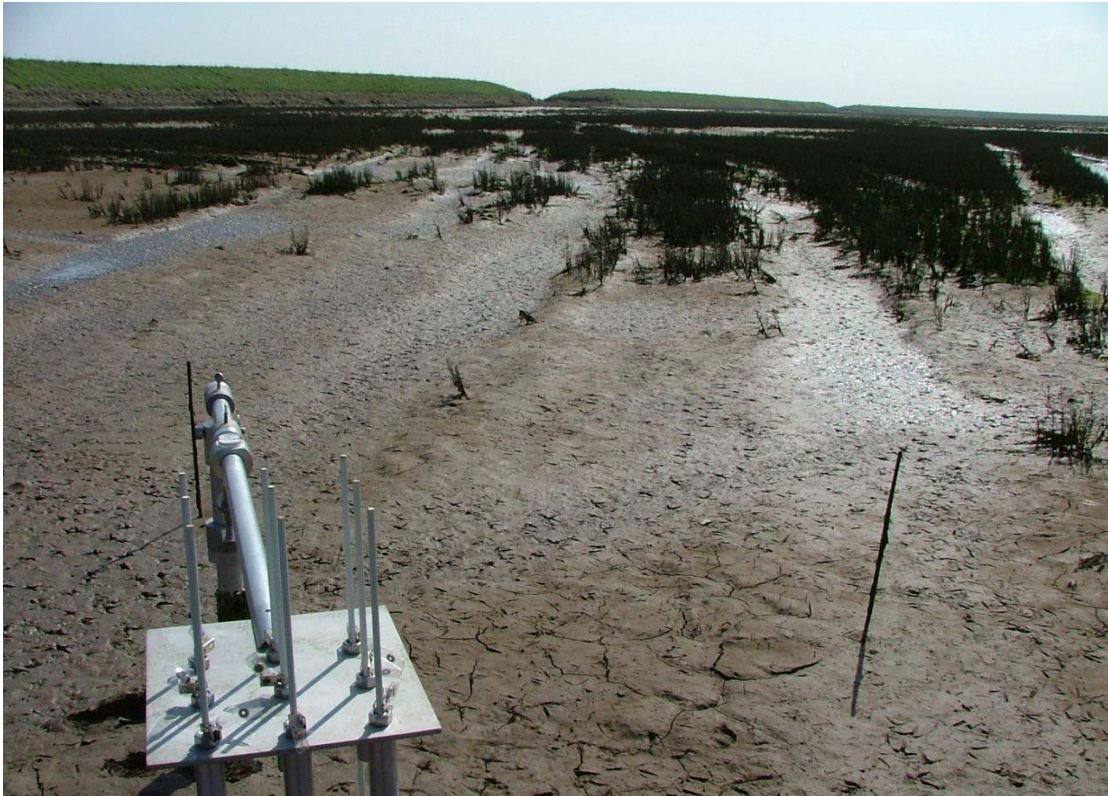
Plate 4.2. SET instrument deployed at site 7 (category: inside the managed realignment, close to the breaches; see Figure 1 for exact location), April 2005. Note less consolidated sediments infilling unvegetated former runnels at this site (photograph: S. Boreham).
