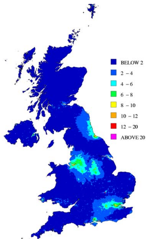
Figure 3.5(d) NETCEN Estimated annual mean background \text{SO}_2 concentration for 2020 ( \mu\text{g m}^{-3} )
