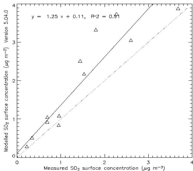
Fig. 3.4 Modelled \text{SO}_2 concentrations for the year 2002 compared with measurements for the period 2001-03
