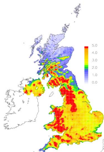
Figure 4.2(f) FRAME 2002 NH x wet deposition (kg N ha -1 )
