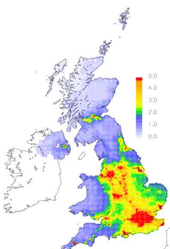
Figure 4.2(c) FRAME 2002 NO y dry deposition (kg N ha -1 )
