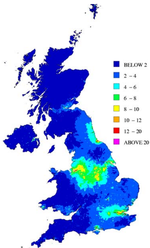
Figure 3.5(c) NETCEN Estimated annual mean background \text{SO}_2 concentration for 2003 ( \mu\text{g m}^{-3} )
