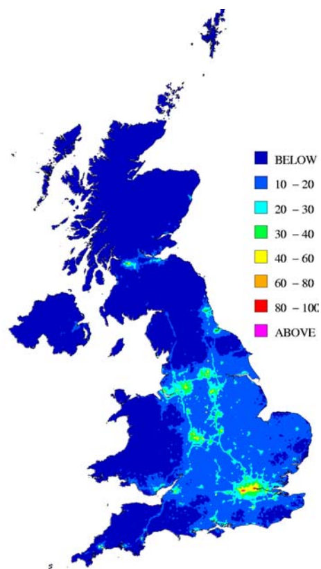
Figure 3.5(b) NETCEN Estimated annual mean background \text{NO}_x concentration for 2020 ( \mu\text{g m}^{-3} )
