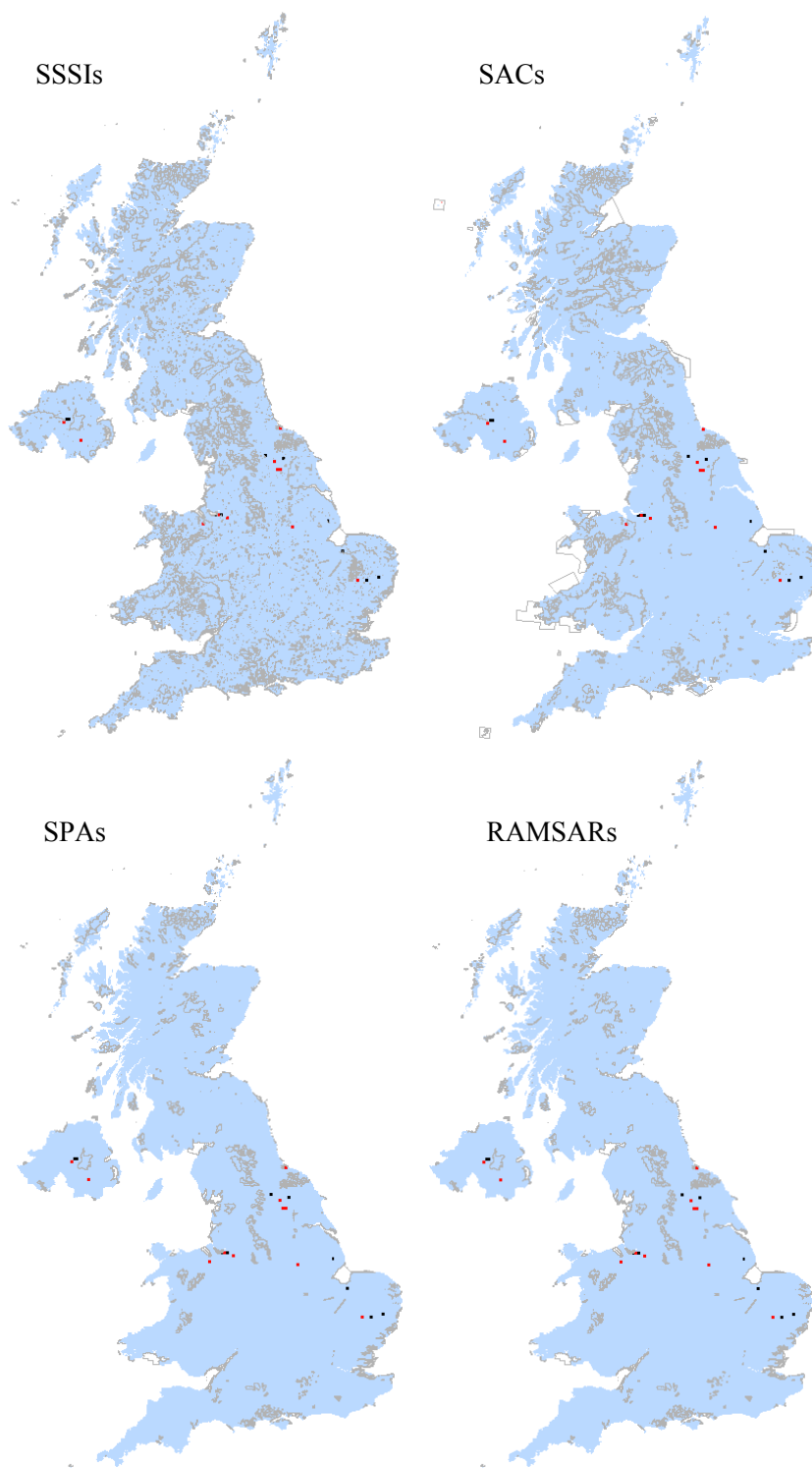
Figure 5.2 Designated areas overlaid on FRAME uncalibrated \text{NH}_3 concentrations: Pale blue: < 8\mu\text{g m}^{-3} in 2002 and 2020 Red: > 8\mu\text{g m}^{-3} in 2002 Black: > 8\mu\text{g m}^{-3} in 2002 and 2020
