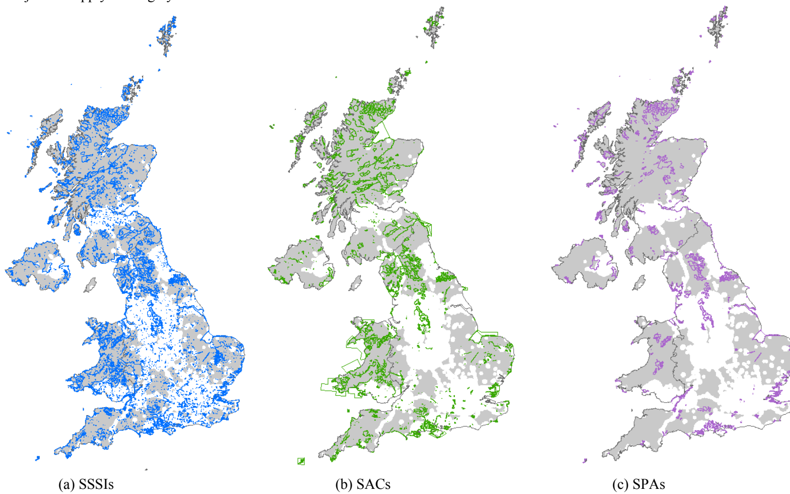
Figure 5.1 Designated areas overlaid on the “exclusion zone” (white areas). Objectives apply in the grey areas
