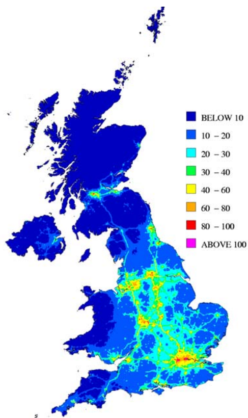
Figure 3.5(a) NETCEN Estimated annual mean background \text{NO}_x concentration for 2003 ( \mu\text{g m}^{-3} )
