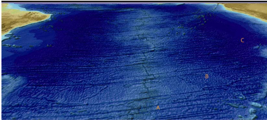
Figure 3. An oblique view of the mid-ocean ridge on the South Atlantic. The detail show in the area immediately to the west of “A” indicates that this area has been mapped with a multibeam bathymetry system, whereas the more generalised topography exhibited around “B” suggest this has mostly been surveyed using single beam echo-sounders. Around area “C” there is what is often described as an “orange-peel” texture (much easier to see on a screen than in print), which indicates (usually over areas of abyssal plain) that here predicted depths from satellite altimetry are used.
