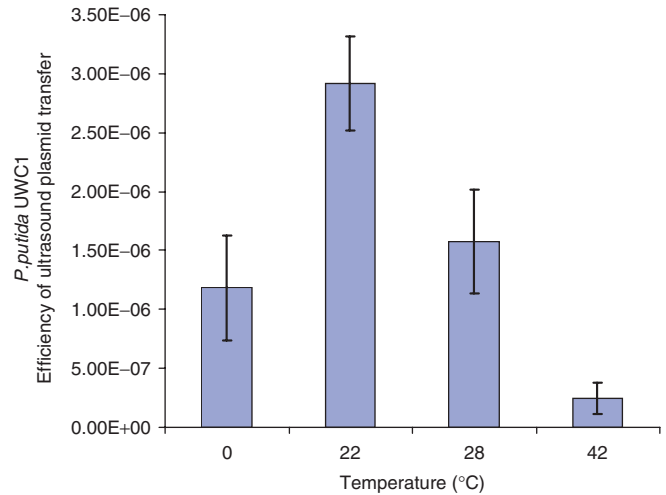
Figure 5. Temperature effect on UDD efficiency of P. putida UWC1. UDD at 22°C gave the highest efficiency ( P < 0.05 ).
