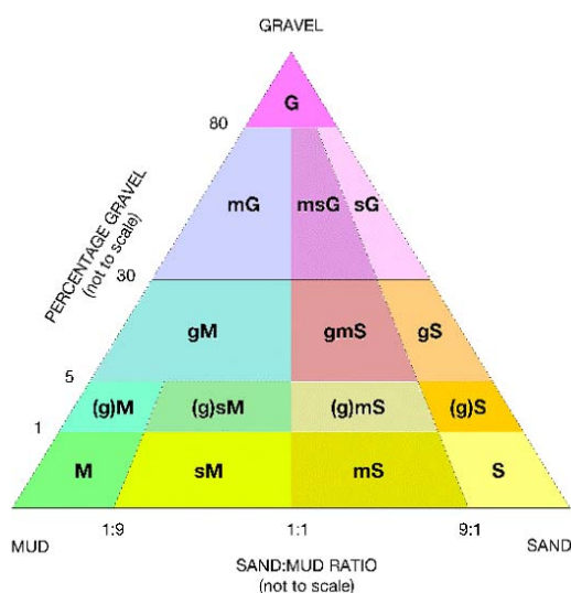
Figure F2 Classification of sea-bed sediments (modified after R L Folk, 1954, Journal of Geology, 62, 344-359)
