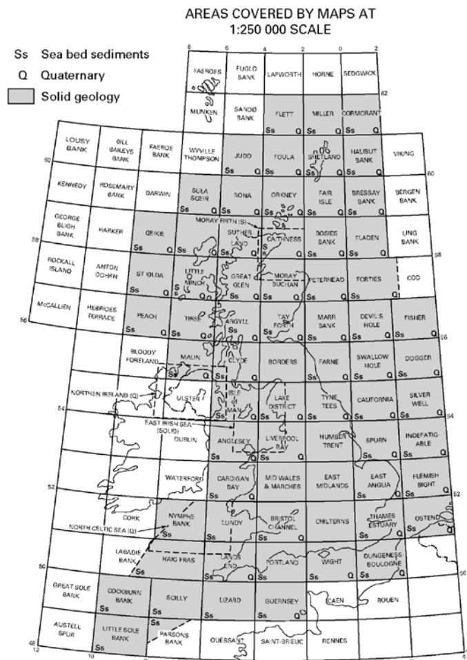
Figure F-1 Distribution of offshore geology maps.
