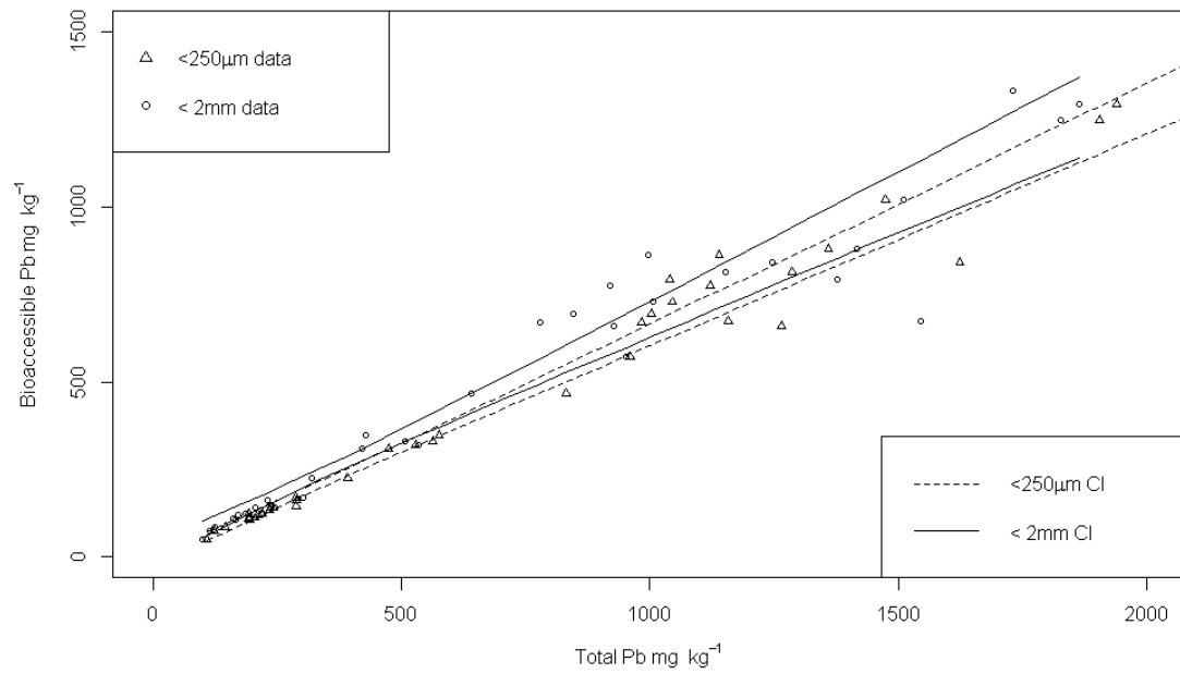
Figure 5 Scatterplot for relationship between total Pb in <2mm and <250 micron fractions and bioaccessible Pb in <250 µm fraction of London topsoils with <2000 mg/kg total Pb.
