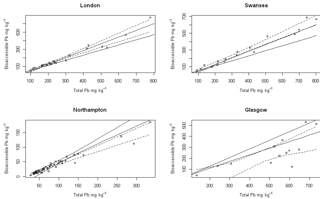
Figure 2 Scatterplot for relationship between total Pb (<2mm fraction) and bioaccessible Pb (<250 micron fraction): <2000 mg kg -1 Pb subset for London Swansea, Northampton and Glasgow. Solid lines show the 95 th percentile confidence limits for all data combined and dotted lines show the 95th confidence interval for the individual data sets
