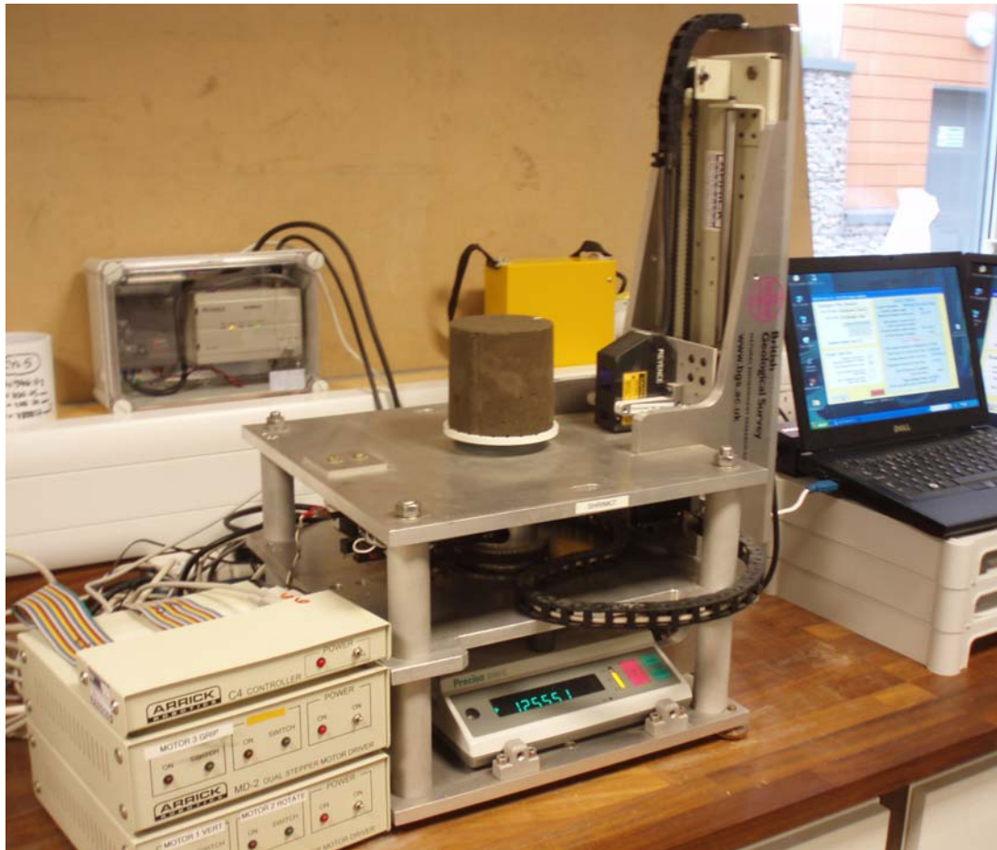
Figure 6 Shrinkage limit apparatus [version 2: fully automated, 'SHRINKiT'] 2012
