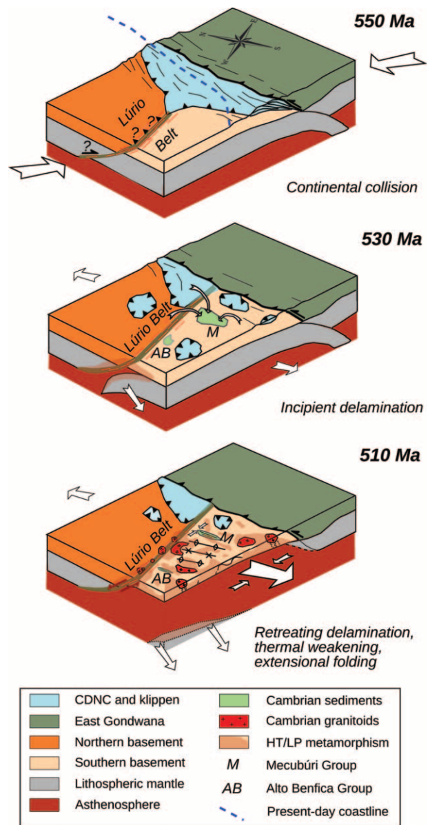
Figure 13. Channellock diagrams showing the evolution of the East African–Antarctic Orogen in northeast Mozambique. The northern and southern basements are part of West Gondwana. Oblique collision with East Gondwana culminated at 550 Ma, emplacing nappes with granulite-facies rocks in a northwesterly direction. The onset of extensional collapse between ca. 540 and 530 Ma exhumed the southern basement and lead to deposition of the Mecubúri and Alto Benfca groups in restricted (Cambrian) sedimentary basins. High-temperature-low-pressure (HT-LP) metamorphism, voluminous granitoid magmatism, and coeval extensional shear along the Lúrio Belt at or slightly before ca. 510 Ma probably dates culmination of thermal and mechanical response to delamination. The Lúrio Belt underwent protracted activity, although the kinematics have not been fully resolved kinematics (red lines show general activity).
