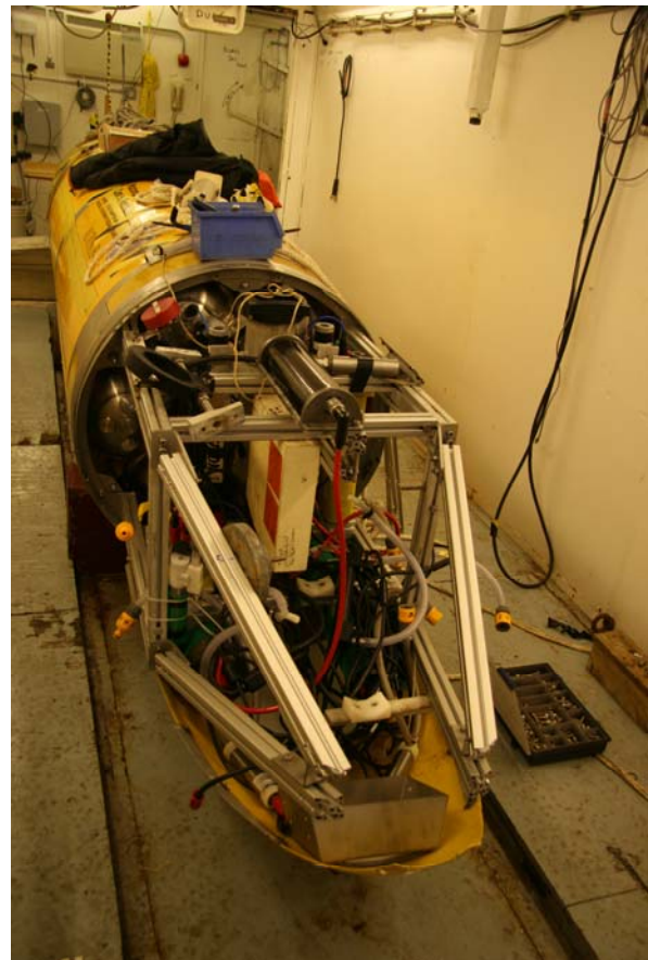
Figure 6 Autosub3 getting reading for mission 432, under the Pine Island Glacier
