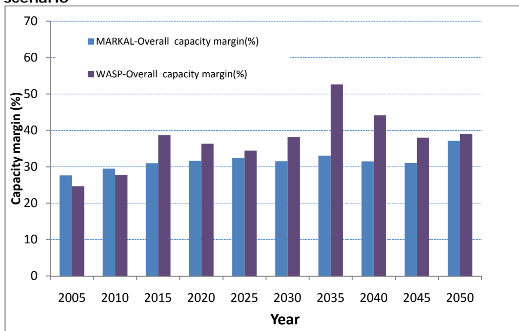
Figure 12: Capacity margin using different reliability approaches, Low-Carbon scenario
