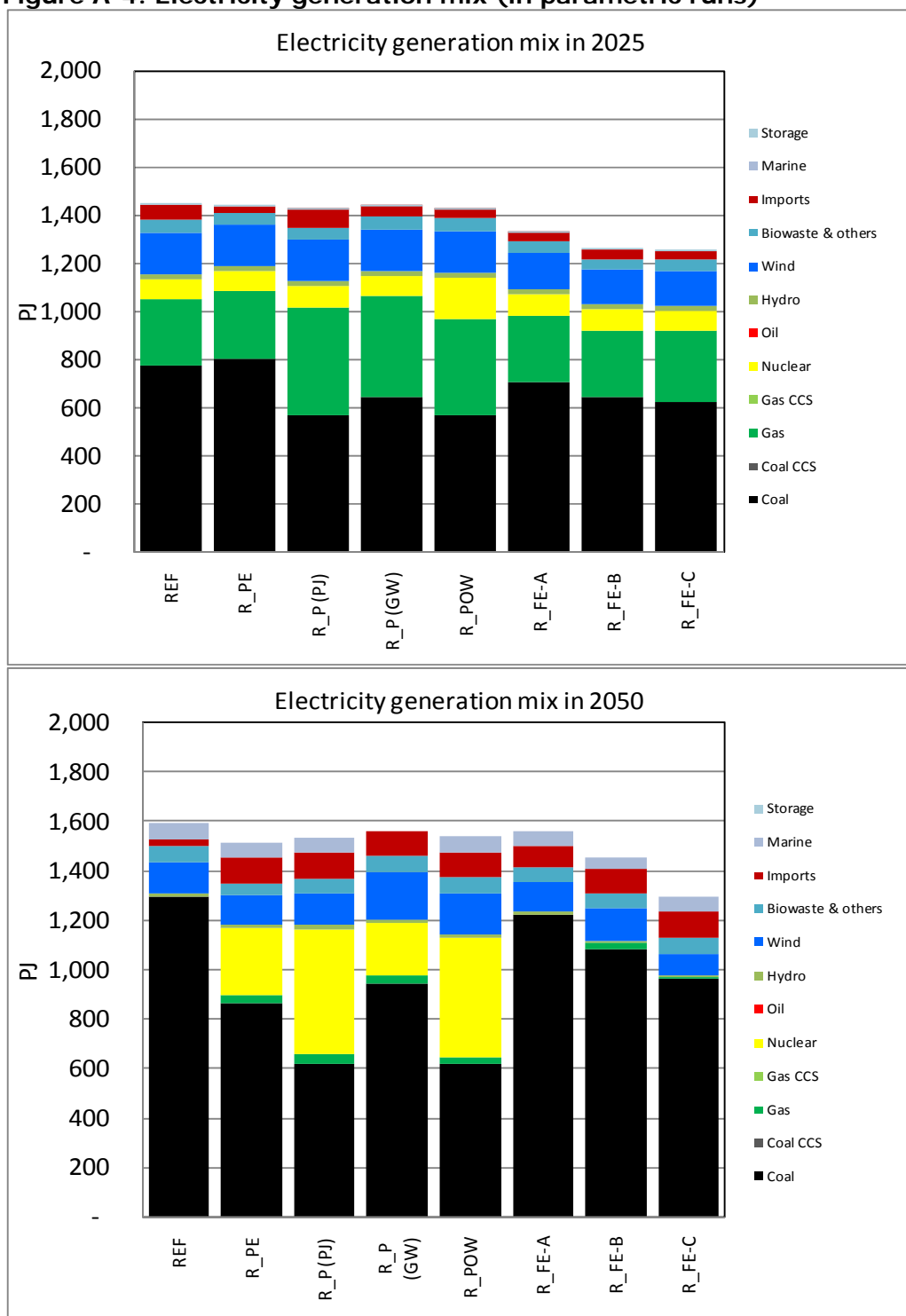
Figure A-4: Electricity generation mix (in parametric runs)
