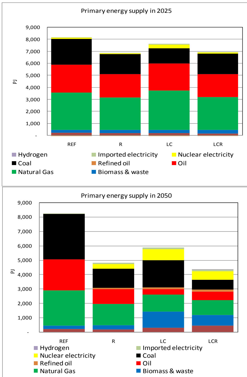
Figure B-2: Primary energy supply in core scenarios
