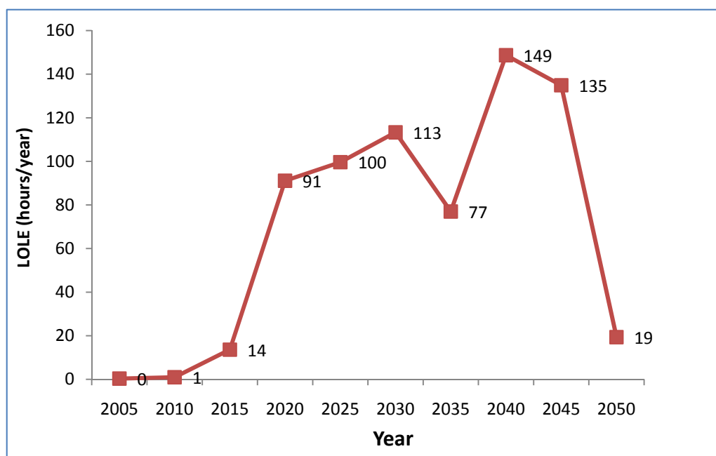
Figure 13: Loss-of-load expectation using capacity margin approach, Low Carbon scenario
