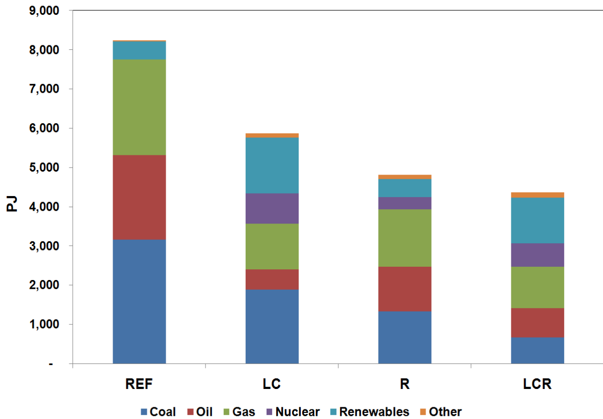
Figure 10: Primary Energy Demand in 2050
