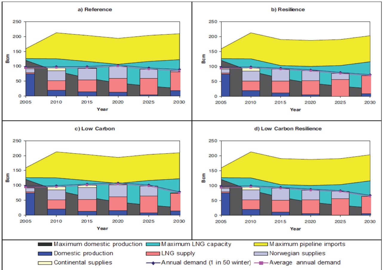
Figure 14: gas supply/demand balance in the four core scenarios
