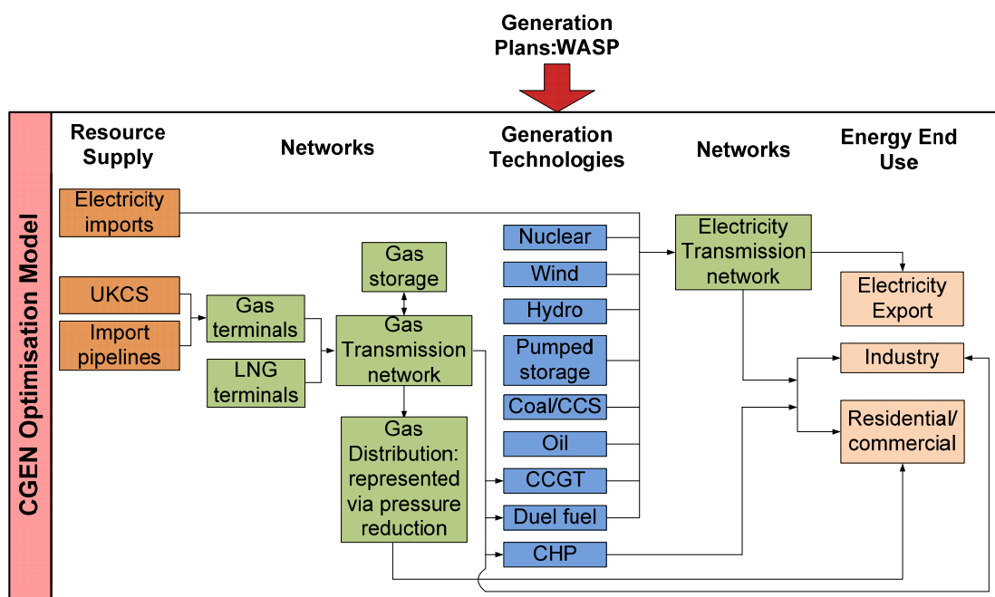
Figure 6. CGEN optimisation model
