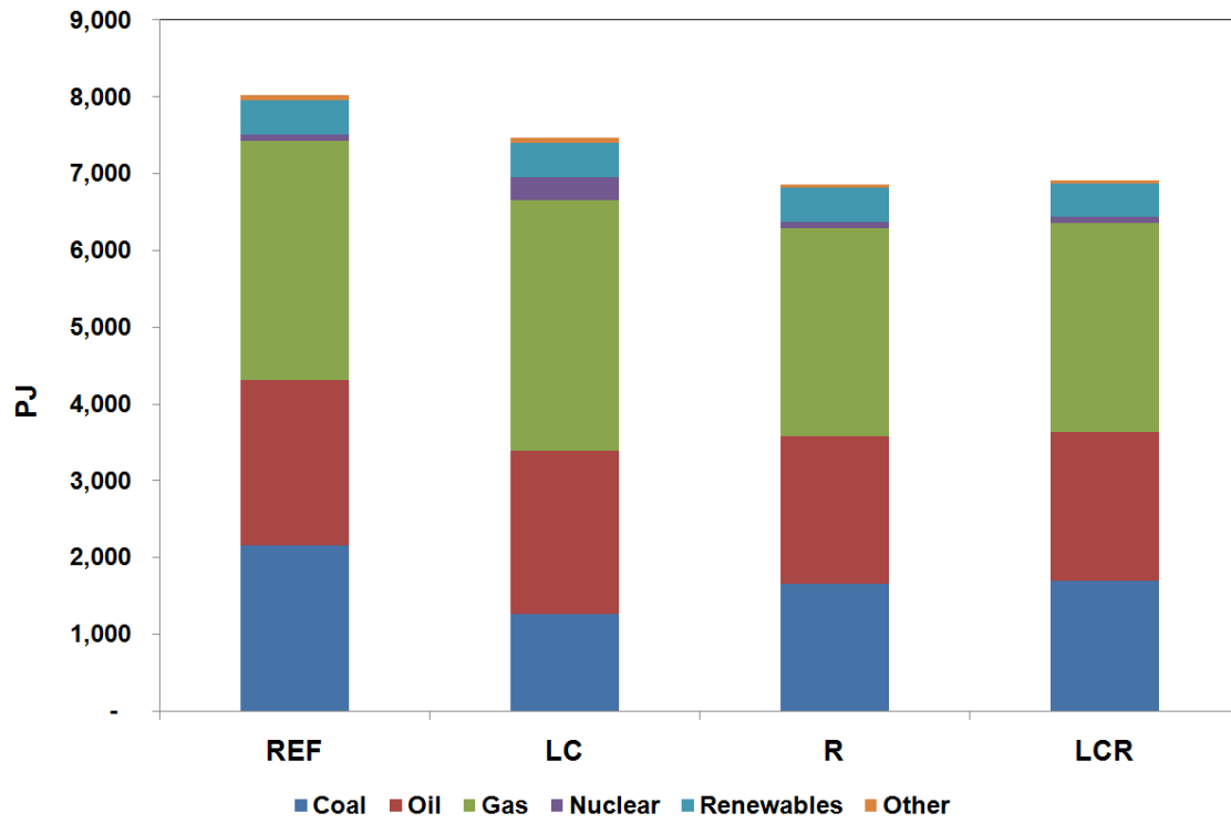
Figure 10: Primary Energy Demand in 2050
