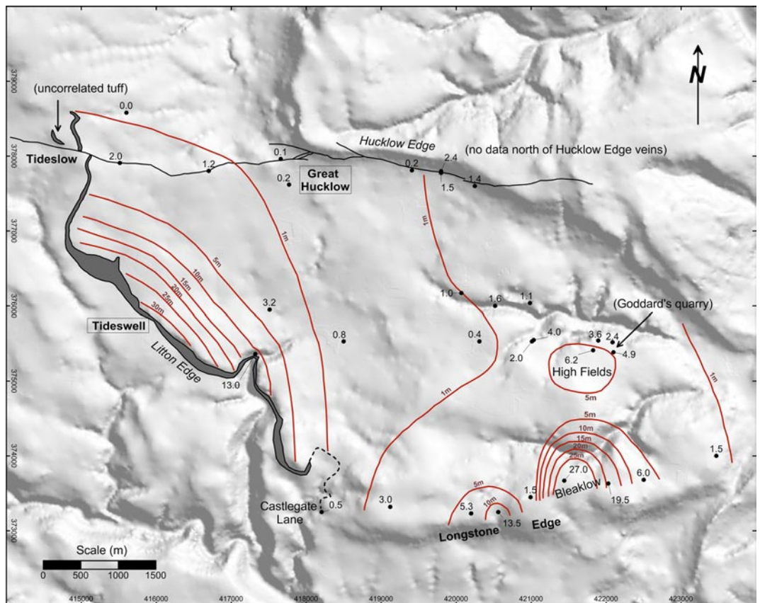
Figure 6. Thicknesses of the Litton Tuff, indicated by isopachytes drawn at 5m intervals.
